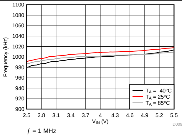
图 10. Backlight Boost Frequency
