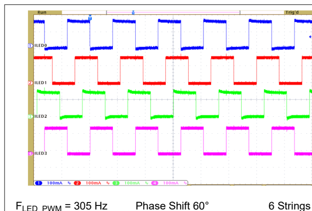
Figure 8-3. LED String Currents Showing Phase Shift PWM Operation
