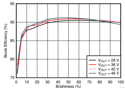
System Efficiency
