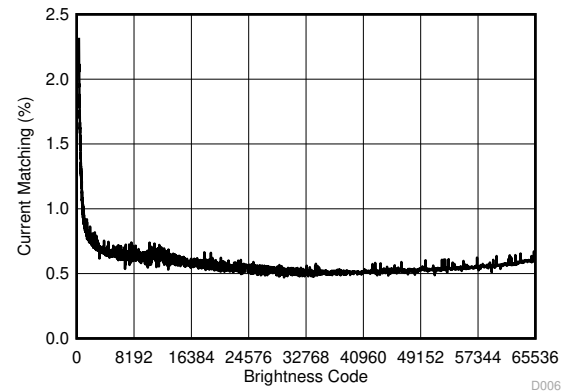
Figure 6-7. Current Matching
