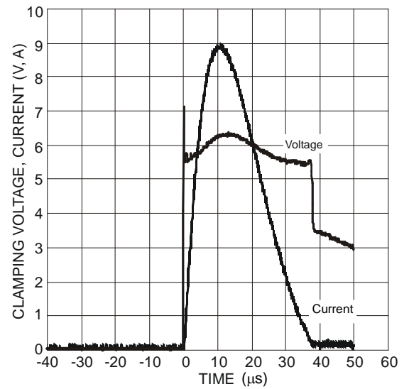
Figure 6 Waveform of Clamping Voltage, Current vs. Time (8/20 \mu s , V_{CC} to V_{SS} )
