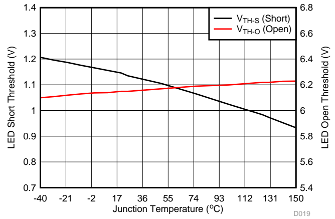
Figure 8. Channel Open and Short Protection Thresholds vs Junction Temperature
