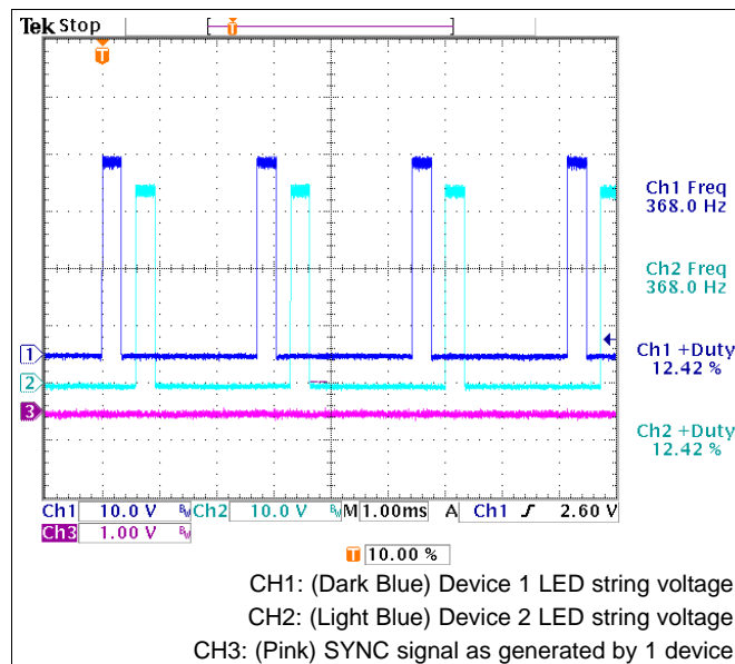
Figure 13. Non-Synchronized TPS92661 Devices
