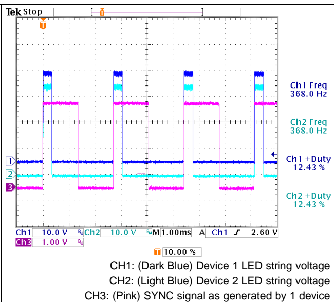
Figure 14. Actively Synchronized TPS92661 Devices
