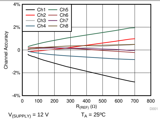
图 8. I_{(IOUTx)} Channel Accuracy vs R_{(REF)}
