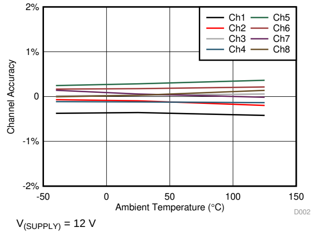
图 2. I_{(IOUTX)} Accuracy vs Ambient Temperature
