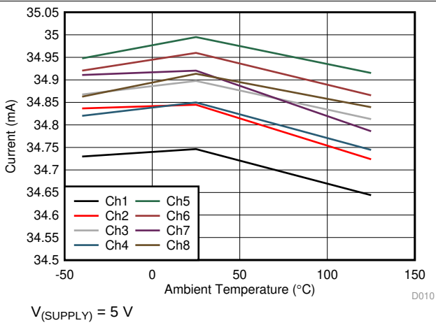
图 4. I_{(IOUTX)} Accuracy vs Ambient Temperature
