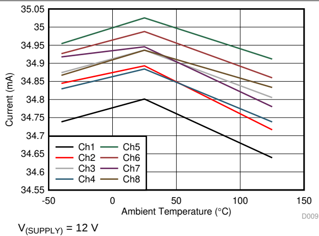
图 3. I_{(IOUTX)} Accuracy vs Ambient Temperature
