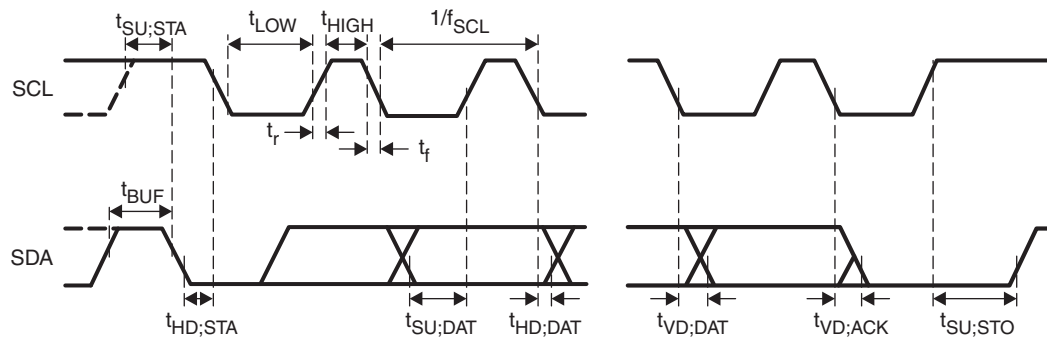
Figure 3. I²C Bus Timing
