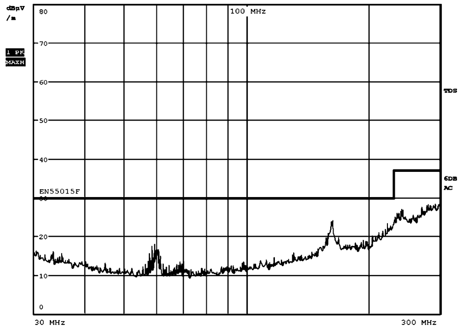
Figure 37. Complies with EN55015 Radiated Emissions (HORI. / HEIGHT=3.0m / RANGE=10m) C IN = 2.2µF, C OUT = 2.2µF, V IN = 60V, I LED = 350mA, No. of LED = 16
