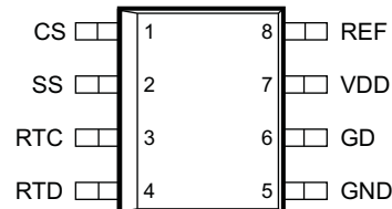
D Package (Top View)
