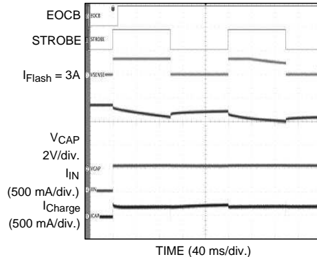
Figure 66. Level-Sensitive Strobe
