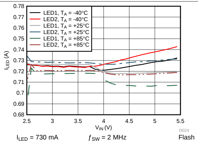
Figure 13. LED1/2 Current vs Input Voltage
