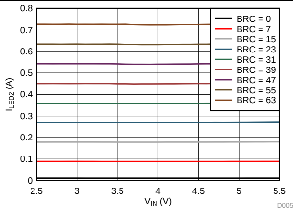
Figure 10. LED2 Current vs Input Voltage
