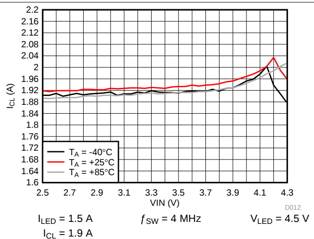
Figure 27. Inductor Current Limit vs Input Voltage
