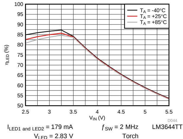
Figure 53. LED Efficiency vs Input Voltage
