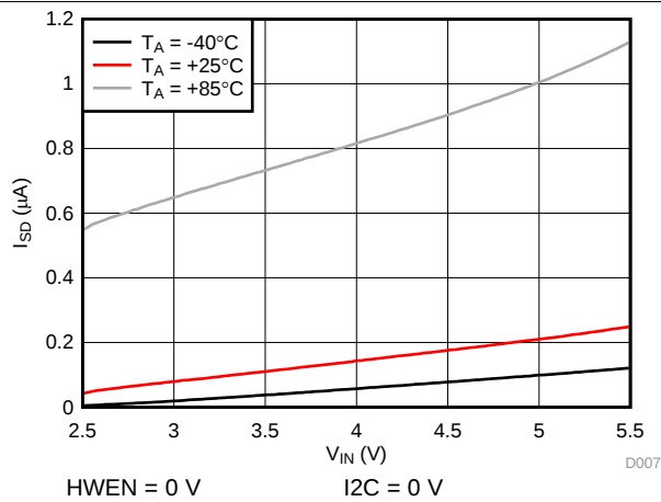
Figure 22. Shutdown Current vs Input Voltage
