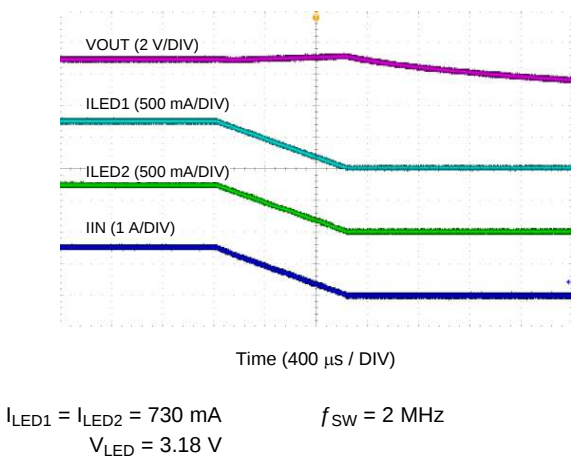
Figure 56. Ramp Down
