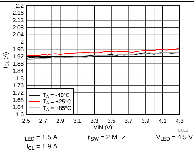
Figure 26. Inductor Current Limit vs Input Voltage
