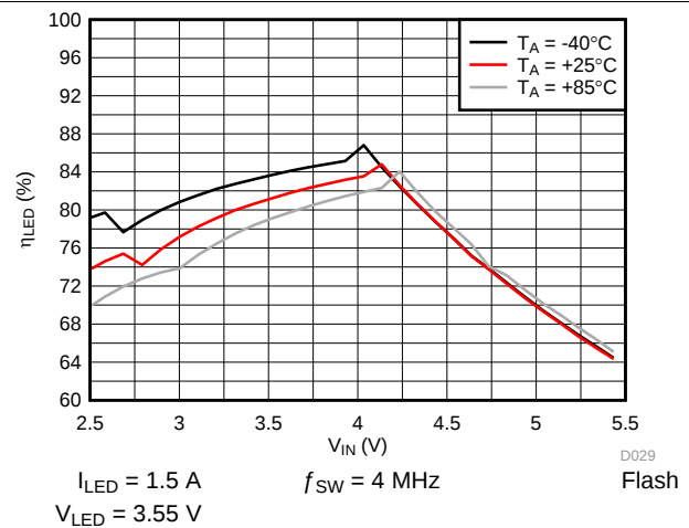
Figure 45. LED Efficiency vs Input Voltage
