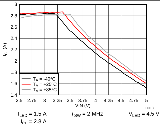
Figure 28. Inductor Current Limit vs Input Voltage
