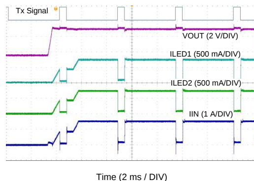
Figure 55. Start-Up
