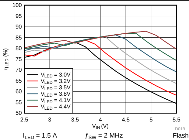
Figure 42. 2-MHz LED Efficiency vs Input Voltage
