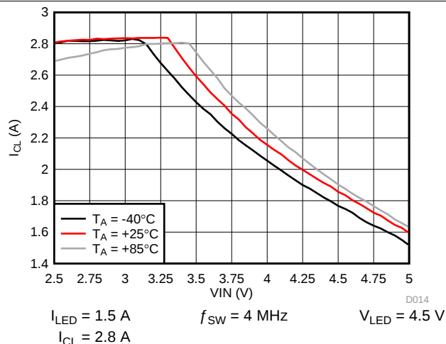
Figure 29. Inductor Current Limit vs Input Voltage
