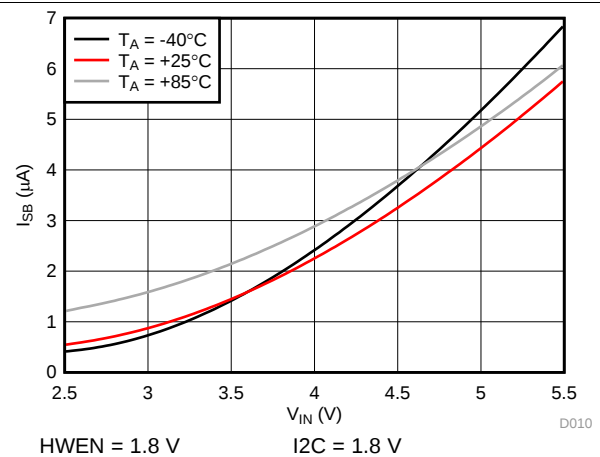
Figure 23. Standby Current vs Input Voltage
