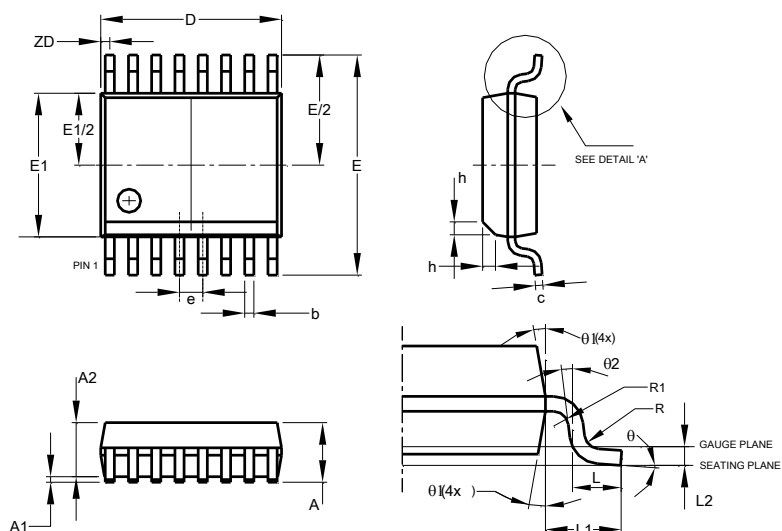
QSOP-16
