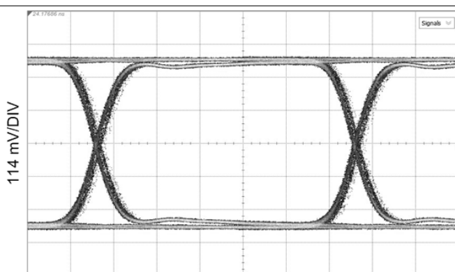
Figure 26. 5.94 Gbps, CC = 120-m Belden 1694A, Reclocked
