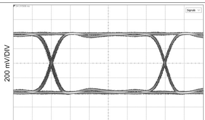
Figure 27. 5.94 Gbps, TL = 20" FR4, Reclocked
