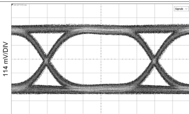
Figure 24. 11.88 Gbps, CC = 75-m Belden 1694A, Reclocked
