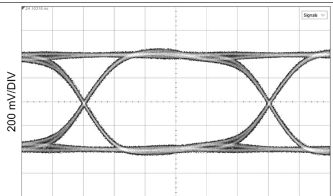
Figure 25. 11.88 Gbps, TL = 20" FR4, Reclocked
