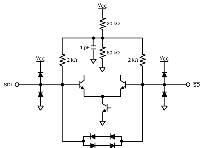
Figure 2. Equivalent SDI input Circuit (SDI, \overline{\text{SDI}} )
