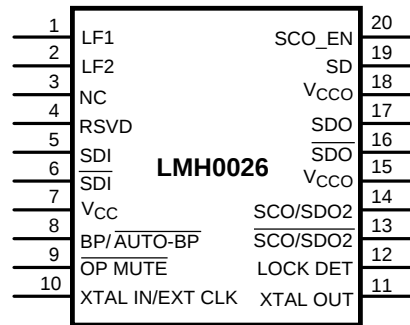
Figure 1. 20-Pin HTSSOP
