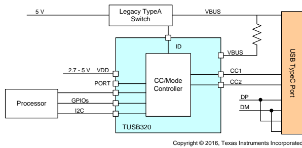
Figure 8. TUSB320 in DRP Mode Supporting Default Implementation
