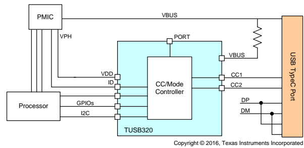
Figure 9. TUSB320 in DRP Mode Supporting Advanced Power Delivery
