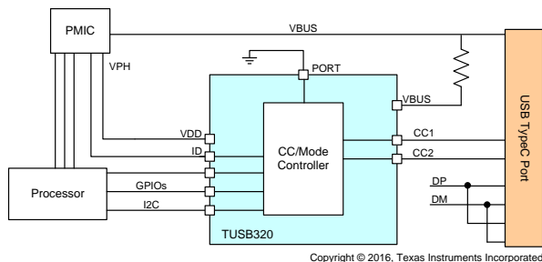
Figure 5. TUSB320 in UFP Mode Supporting Advanced Power Delivery
