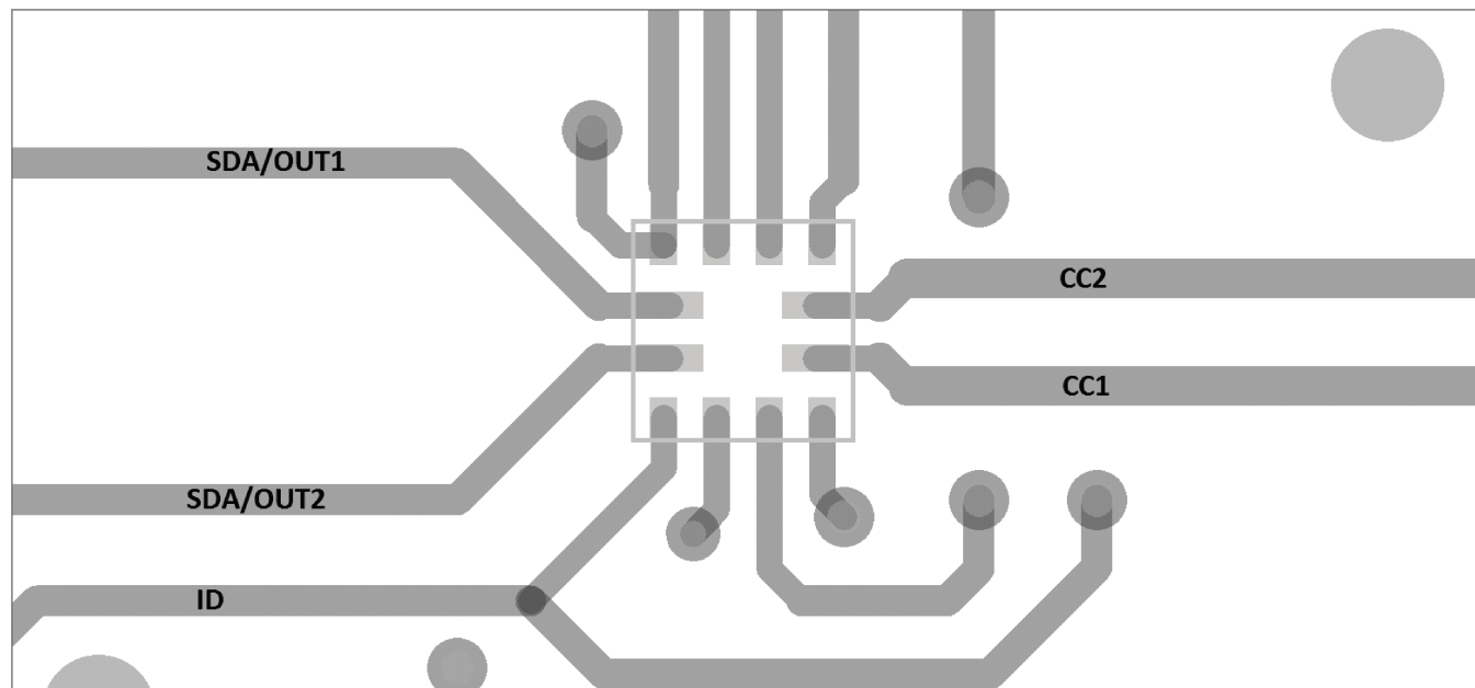
Figure 16. TUSB320 Layout
