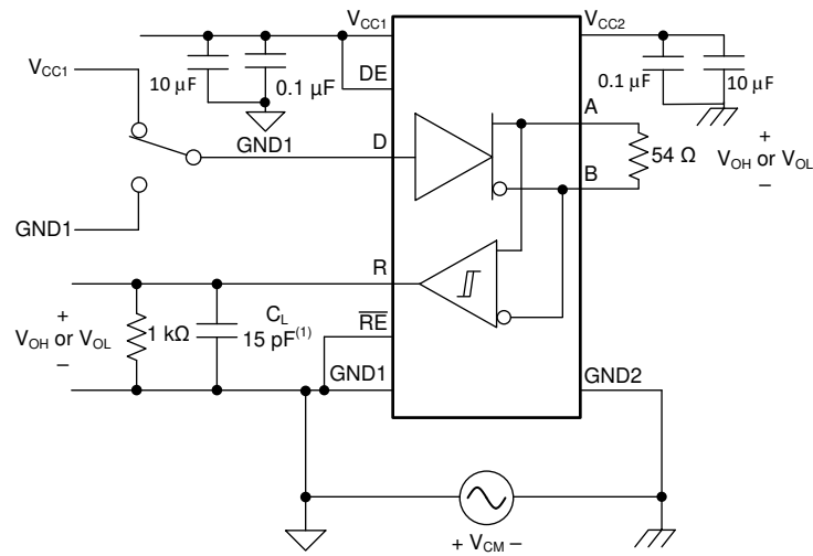
图 39. Common Mode Transient Immunity (CMTI)—Half Duplex
