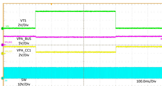
Figure 11-28. OUT Hot Short to GND
