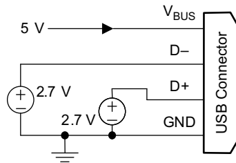
Figure 10-16. Divider 3 Mode
