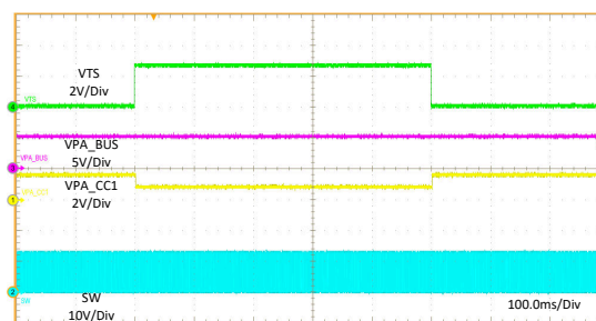
Figure 11-27. OUT short to 5.1- \Omega Load
