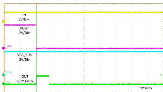
Figure 11-26. PA_CC2 Hot Short to GND
