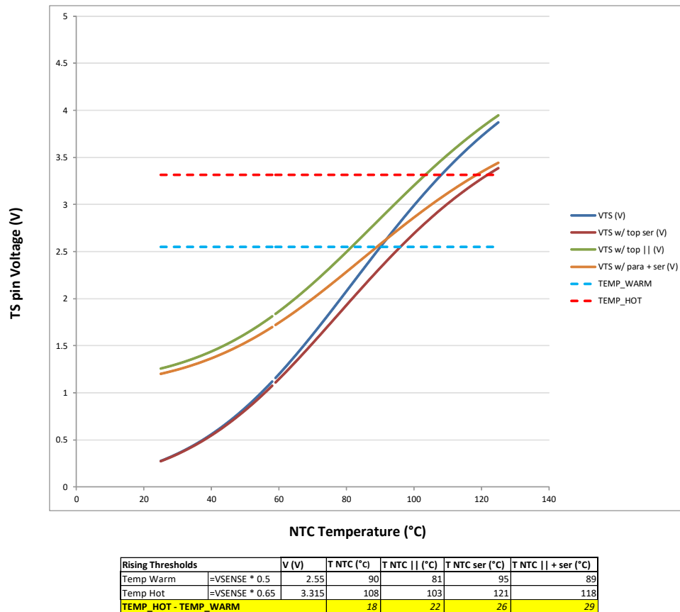
Figure 10-12. V_{\text{TS}} Threshold Design Examples
