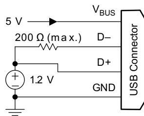
Figure 10-17. 1.2-V Mode
