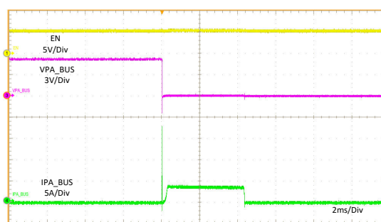
Figure 11-25. VBUS Hot Short to GND
