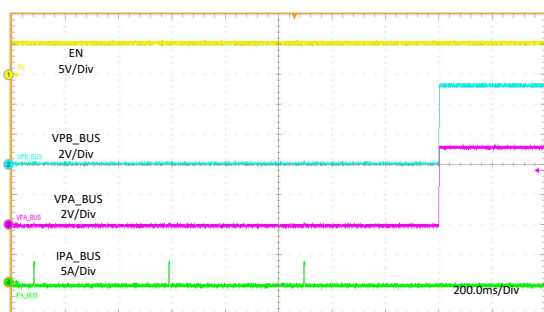
Figure 11-22. Short Circuit Recovery
