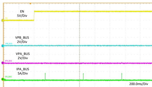
Figure 11-21. Enable Into Short
