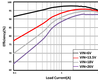
Figure 11-2. Buck Only Efficiency
