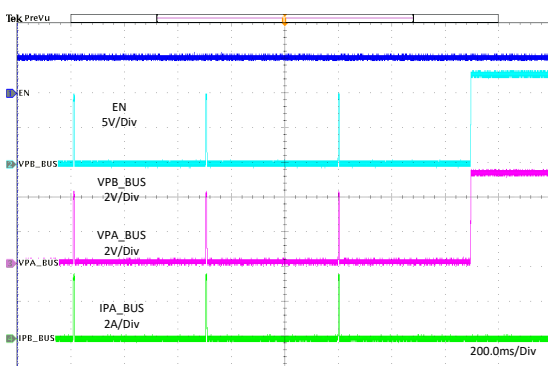
Figure 11-24. 1- \Omega Load Recovery
