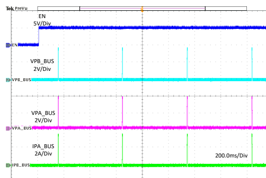
Figure 11-21. Enable Into Short
