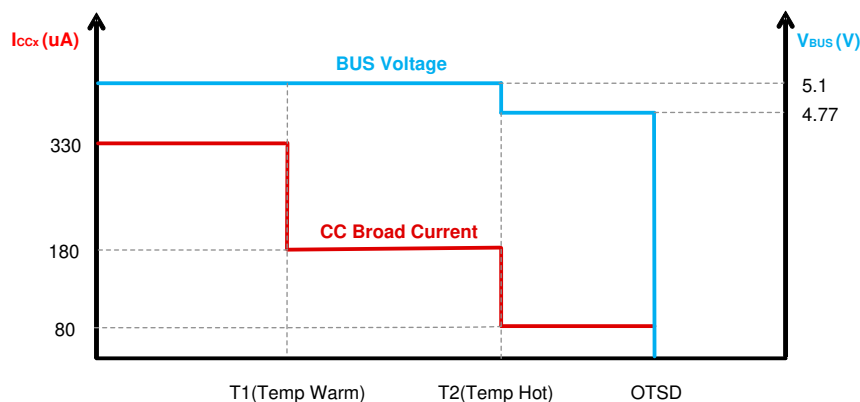
Figure 10-11. TPS25858-Q1 Behavior When Trigger Temp Warm/Hot Threshold
