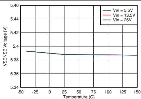
Figure 8-5. V_{SENSE} Voltage vs Junction Temperature
