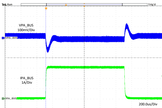
Figure 11-4. Load Regulation
