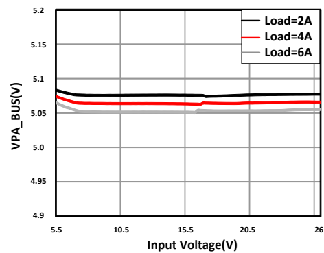
Figure 11-11. Dropout Characteristic
