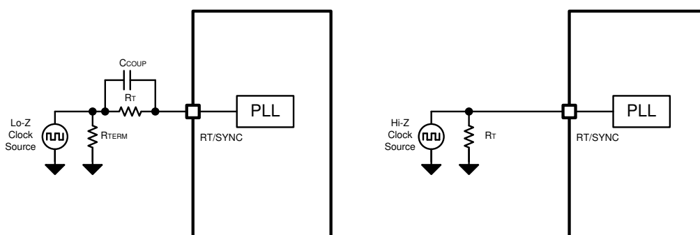
图 44. Synchronize to External Clock
