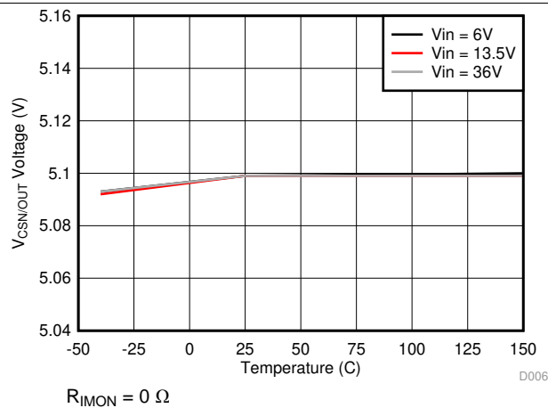
图 7. V_{CSN/OUT} Voltage vs Junction Temperature
