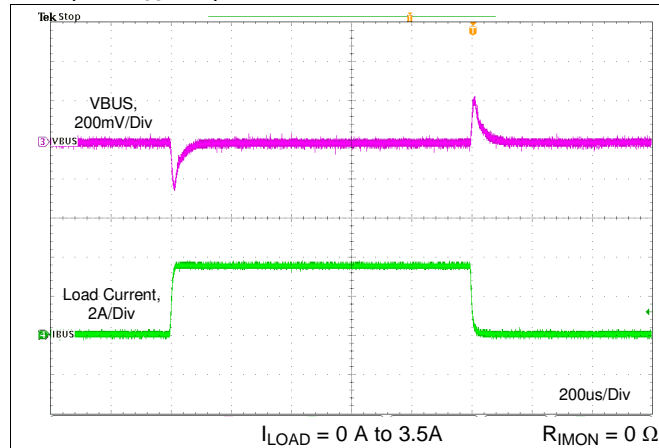
图 80. Load Transient Without Cable Compensation
