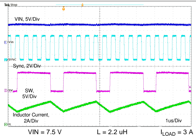
图 48. Synchronizing to External 2.1MHz Clock
