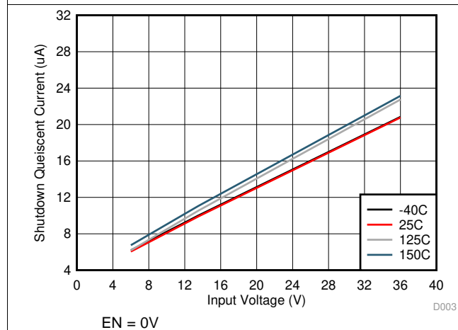
图 3. Shutdown Quiescent Current
