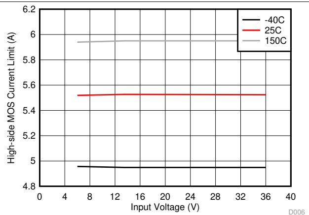
图 8. High-side Current Limit vs Input Voltage
