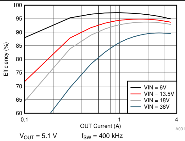
图 74. Buck Only Efficiency
