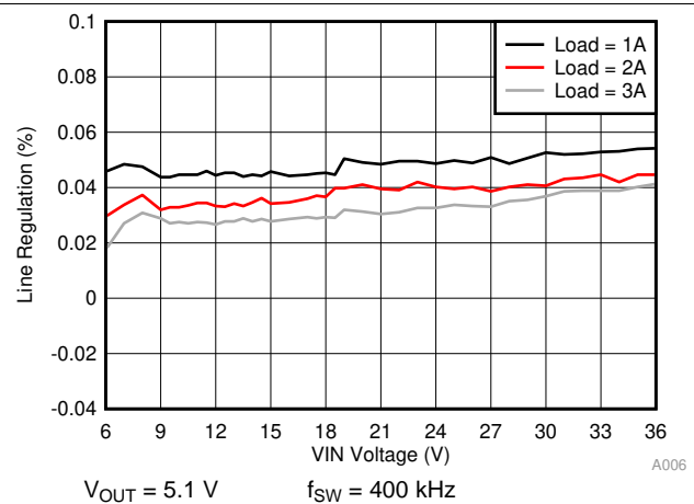
图 79. Line Regulation
