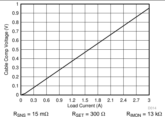
图 18. Cable Compensation Voltage vs Load Current
