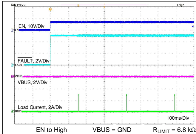
图 98. Enable into Short With External FET
