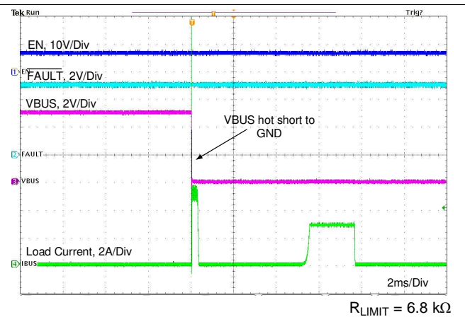
图 101. VBUS Hot Short to GND With External FET
