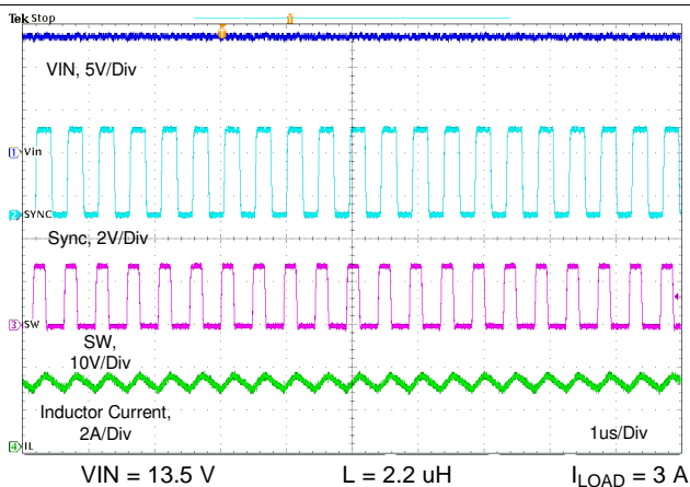
图 49. Synchronizing to External 2.1MHz Clock
