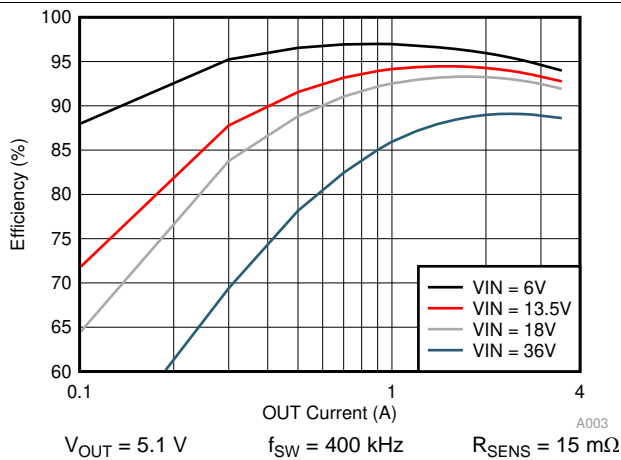
图 76. Efficiency with Sense Resistor
