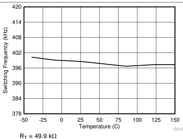
图 11. Switching Frequency vs Junction Temperature
