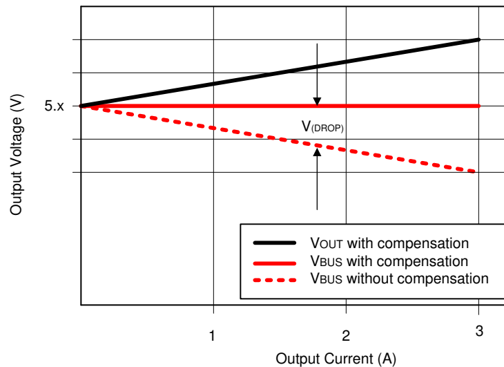
图 60. Voltage Drop
