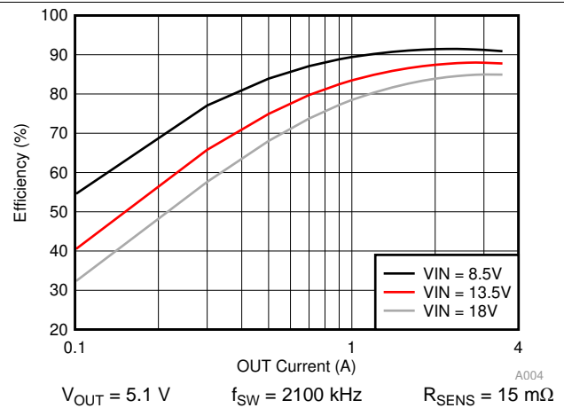
图 77. Efficiency with Sense Resistor
