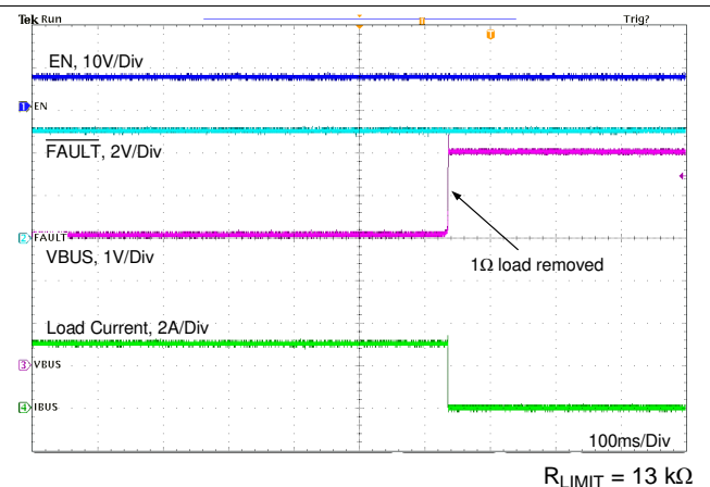
图 97. 1-Ω Load Recovery Without External FET
