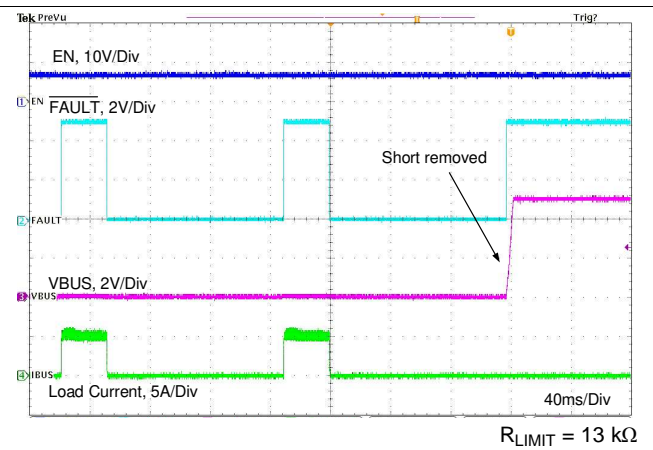
图 95. Short Circuit Recovery Without External FET
