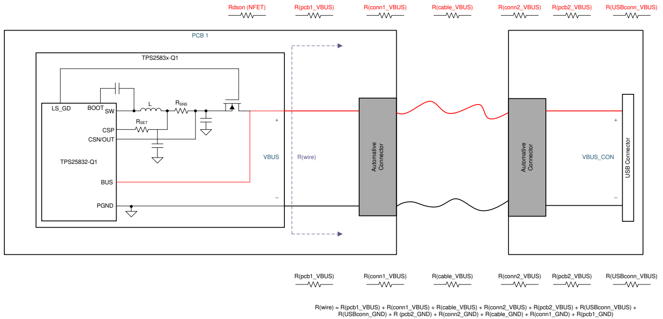
图 59. Automotive USB Resistances
