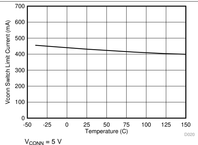
图 24. V_{CONN} Switch Current Limit vs Junction Temperature
