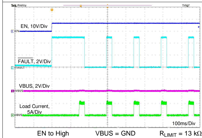
图 94. Enable into Short Without External FET
