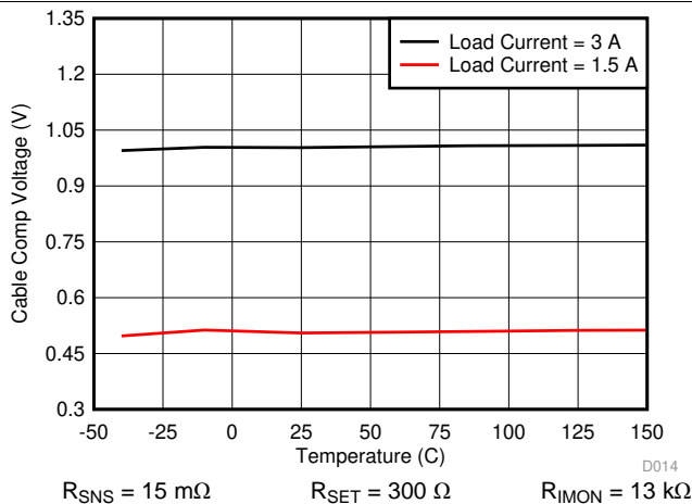
图 17. Cable Compensation Voltage vs Junction Temperature
