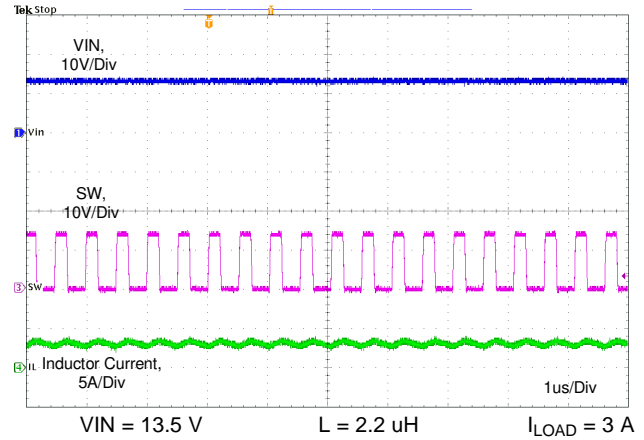
图 46. Switching Frequency when R_T = 8.87 \text{ k}\Omega
