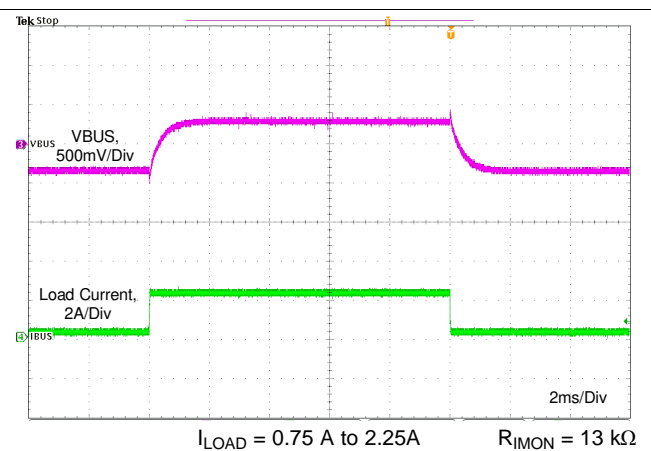
图 83. Load Transient With Cable Compensation
