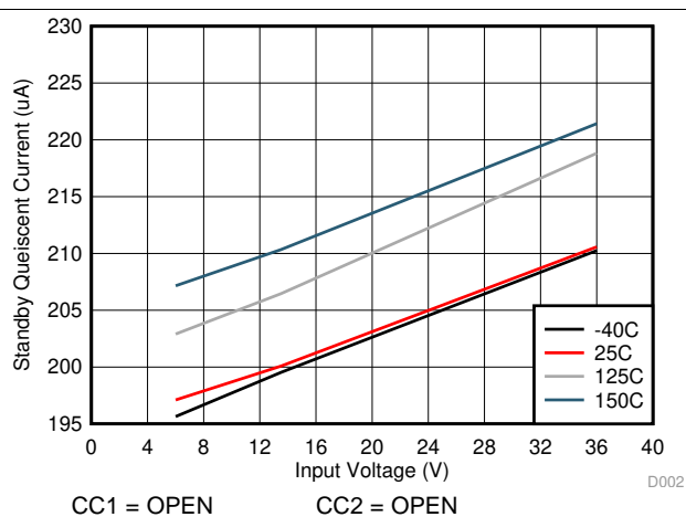
图 2. Standby Quiescent Current
