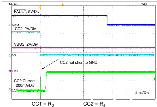
图 102. CC2 Hot Short to GND
