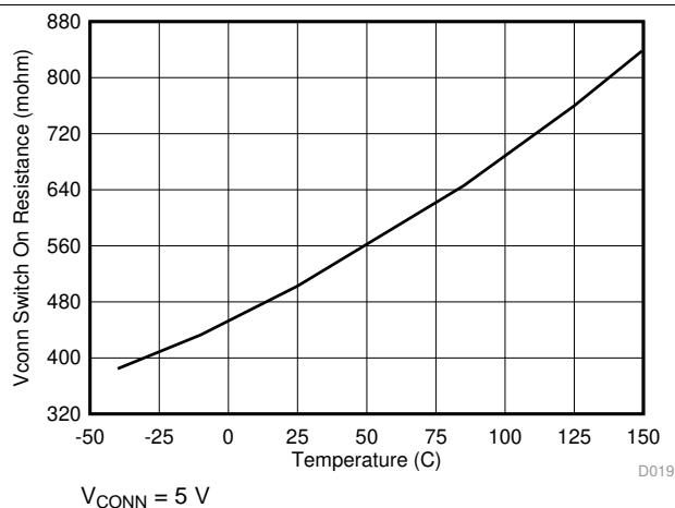
图 23. V_{CONN} Current Limiting Switch On Resistance vs Junction Temperature
