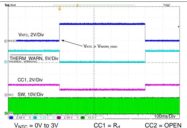
图 103. Thermal Sensing with NTC Behavior 1
