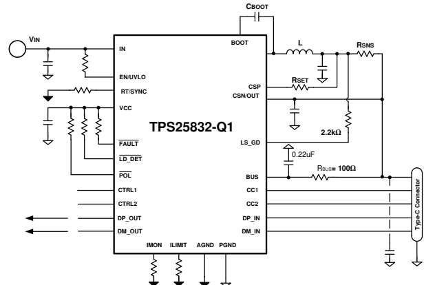
图 58. Buck Average Current Limit
