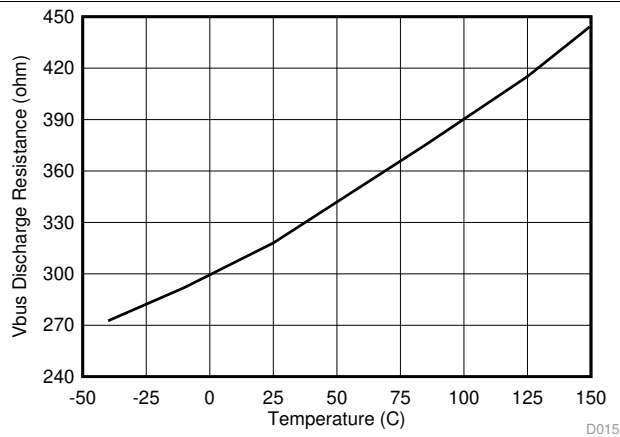
图 19. V_{BUS} Discharge Resistance vs Junction Temperature
