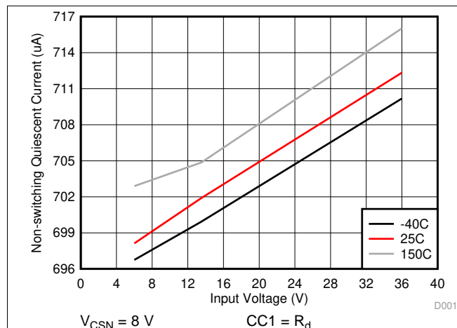
图 1. Non-Switching Quiescent Current
