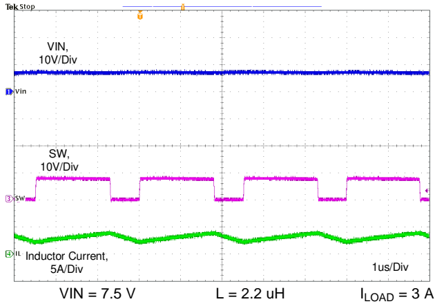
图 45. Switching Frequency when R_T = 8.87 \text{ k}\Omega
