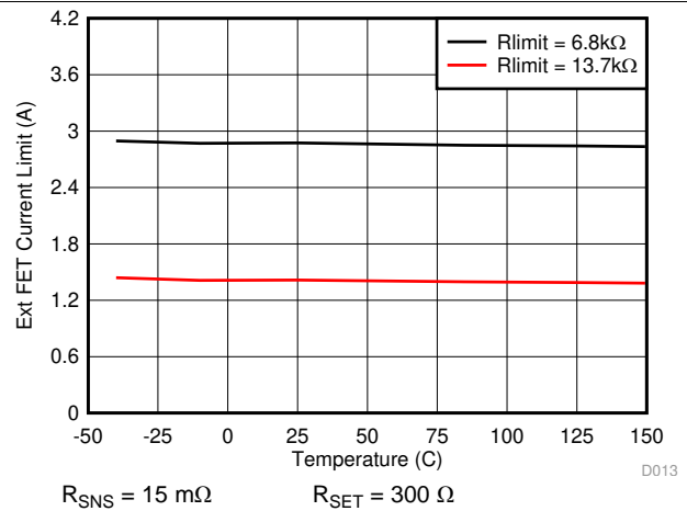
图 14. External FET Current Limit vs Junction Temperature
