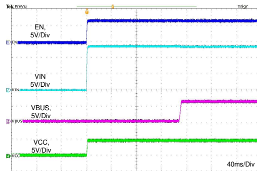
图 41. Typical Start-up Behavior, V_{IN} = 13.5 \text{ V} , CC1 = R_d , R_{IMON} = 12.6 \text{ k}\Omega
