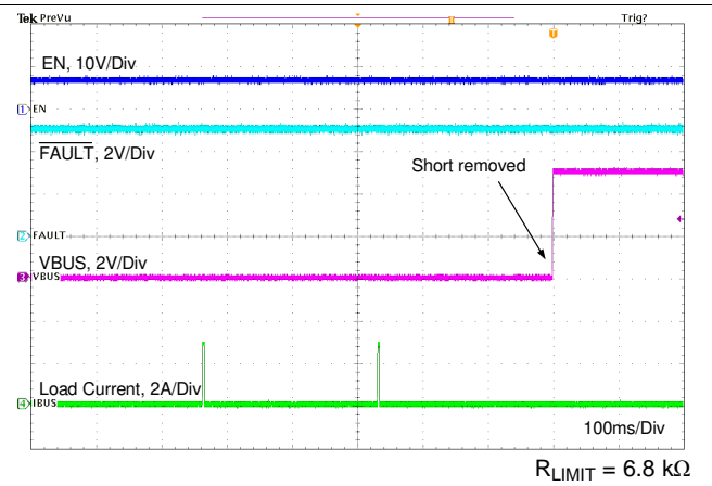
图 99. Short Circuit Recovery With External FET
