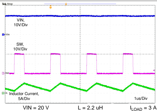
图 47. Switching Frequency when R_T = 8.87 \text{ k}\Omega
