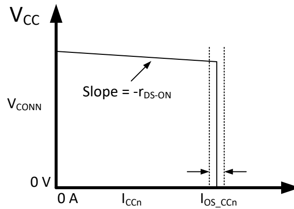
图 63. VCONN Current Limit Profile
