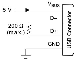
图 69. DCP Supporting BC1.2 and YD/T 1591-2009
