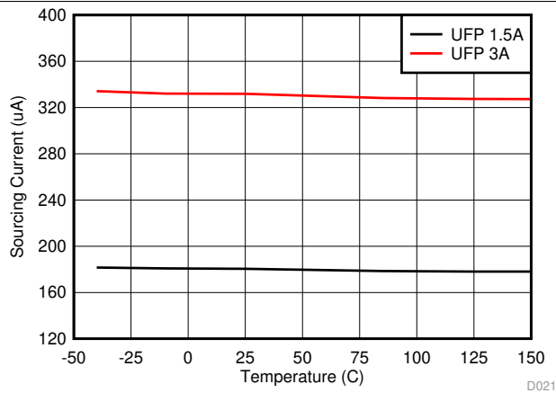
图 25. CC Sourcing Current vs Junction Temperature
