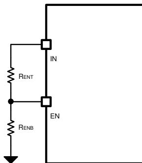
图 40. System UVLO by Enable Divider
