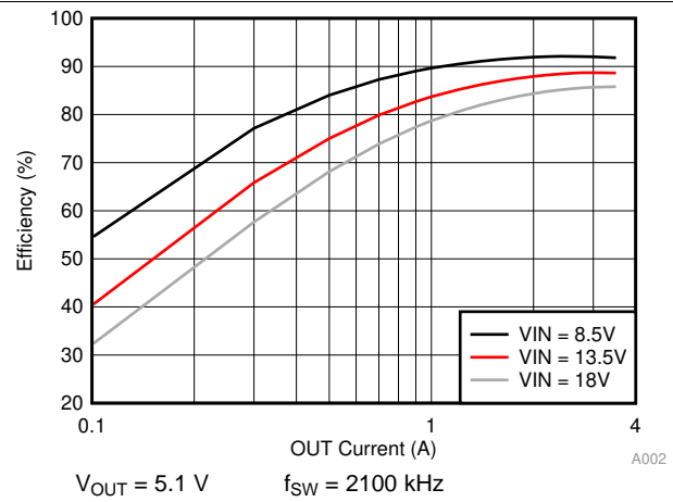
图 75. Buck Only Efficiency
