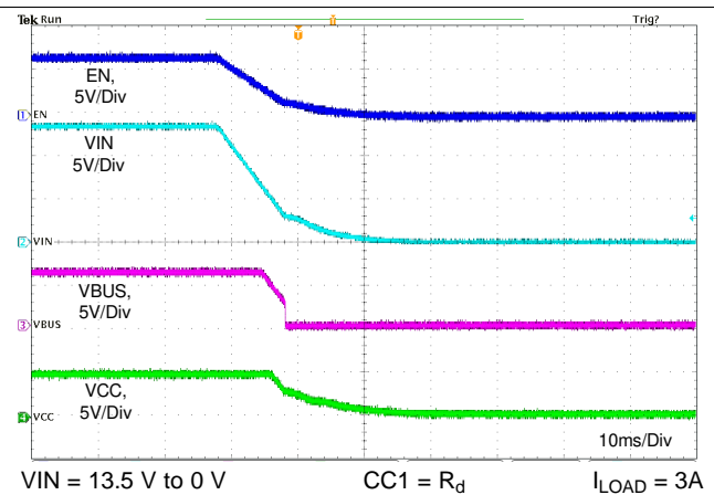
图 89. Shutdown Relate to VIN
