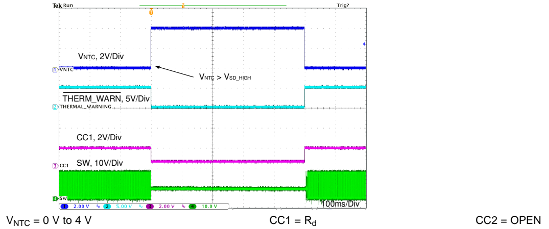
图 104. Thermal Sensing with NTC Behavior 2
