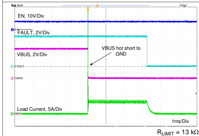
图 100. VBUS Hot Short to GND Without External FET
