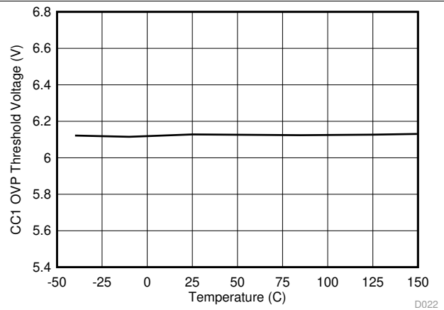
图 26. CC1 Overvoltage Protection Threshold vs Junction Temperature
