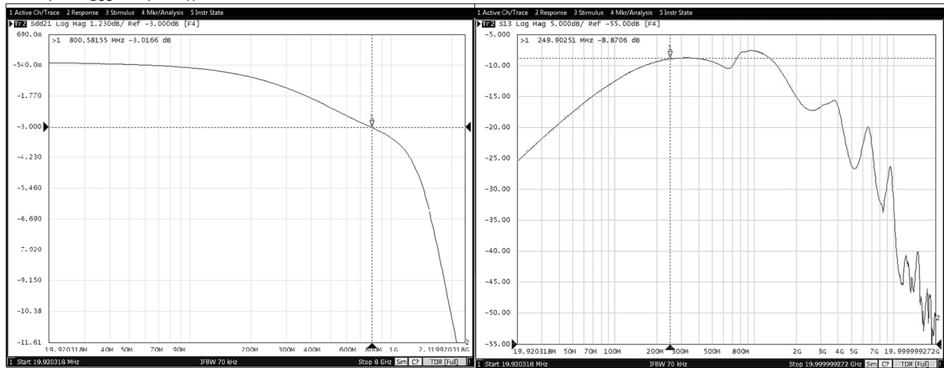
图 31. Data Transmission Characteristics vs Frequency (TPS25832-Q1)
