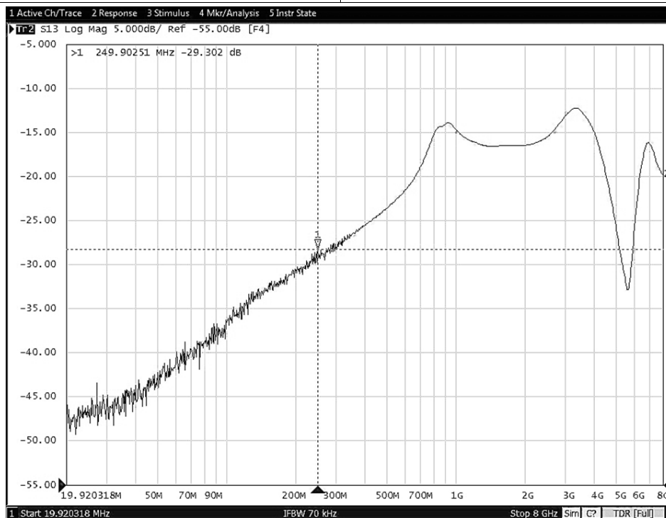
图 32. Off-State Data-Switch Isolation vs Frequency (TPS25832-Q1)
