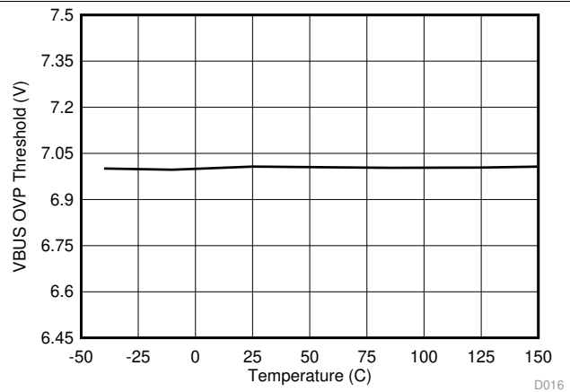
图 20. V_{BUS} Overvoltage Protection Threshold vs Junction Temperature
