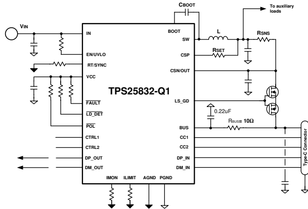
图 57. Current Limit with External MOSFET
