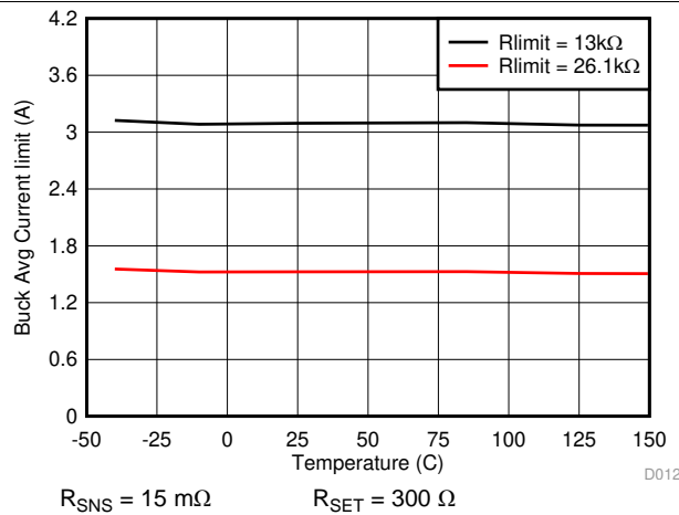
图 13. Buck Average Current Limit vs Junction Temperature
