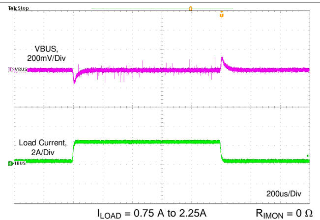
图 81. Load Transient Without Cable Compensation
