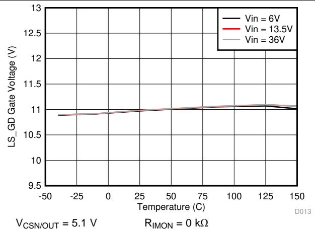
图 16. LS_GD Gate Voltage vs Junction Temperature
