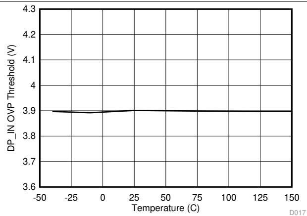
图 21. DP_IN Overvoltage Protection Threshold vs Junction Temperature
