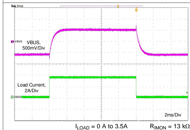
图 82. Load Transient With Cable Compensation
