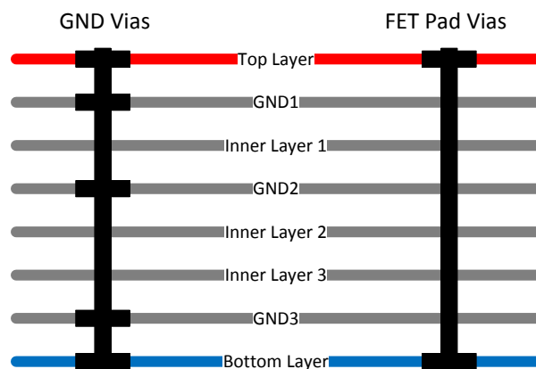
Figure 55. PCB Stack-Up
