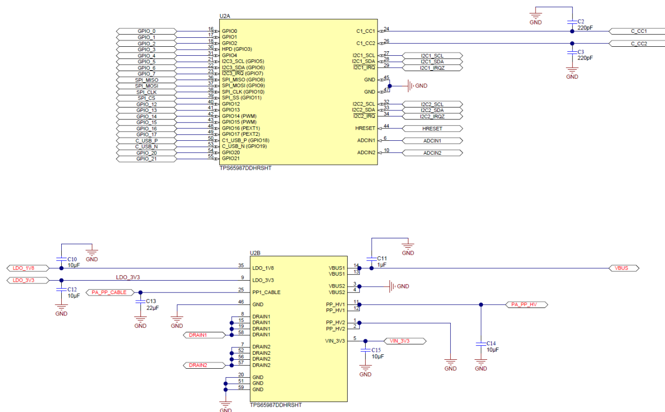
Figure 42. Example Schematic
