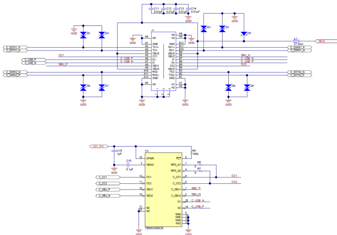
Figure 43. Example Schematic2
