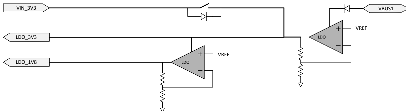
Figure 12. Power Supplies
