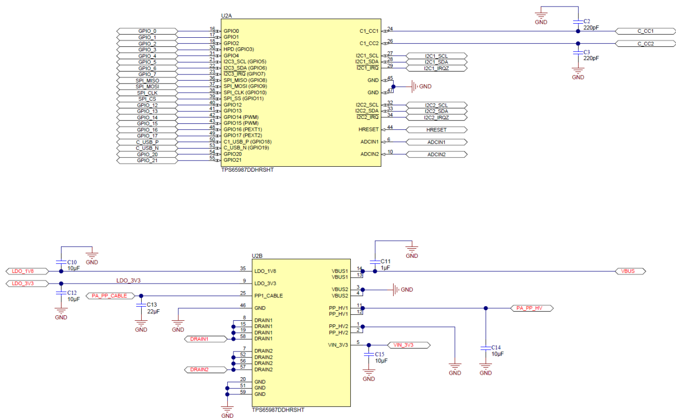
Figure 33. Example Schematic
