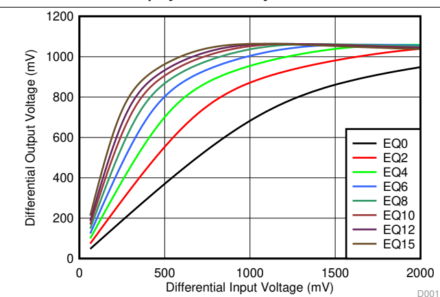
图 4. DisplayPort Linearity Curves at 4.05 GHz
