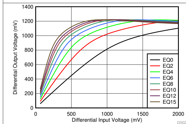
图 3. USB TX (UFP) EQ Settings Curves
