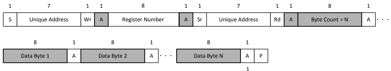
图 31. I 2 C Unique Address Read Register Protocol
