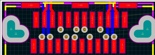
图 50. Type-C Connector Via Placement
