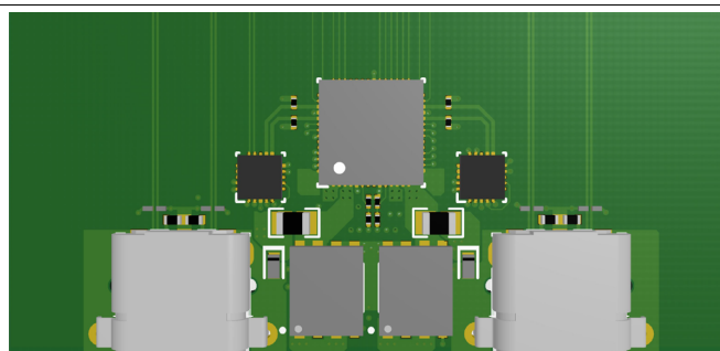
图 71. Top 3D View
