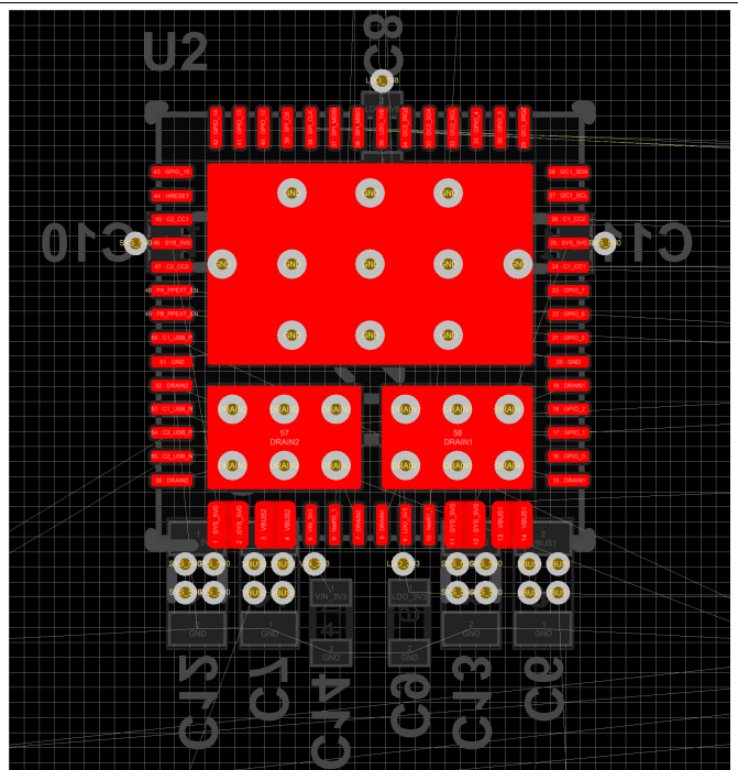
图 54. System Capacitors Placement Top Layer
