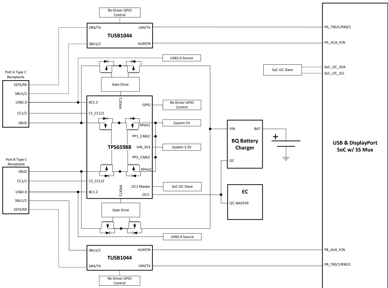
图 42. TPS65988DJ and SoC I2C with Re-Driver GPIO
