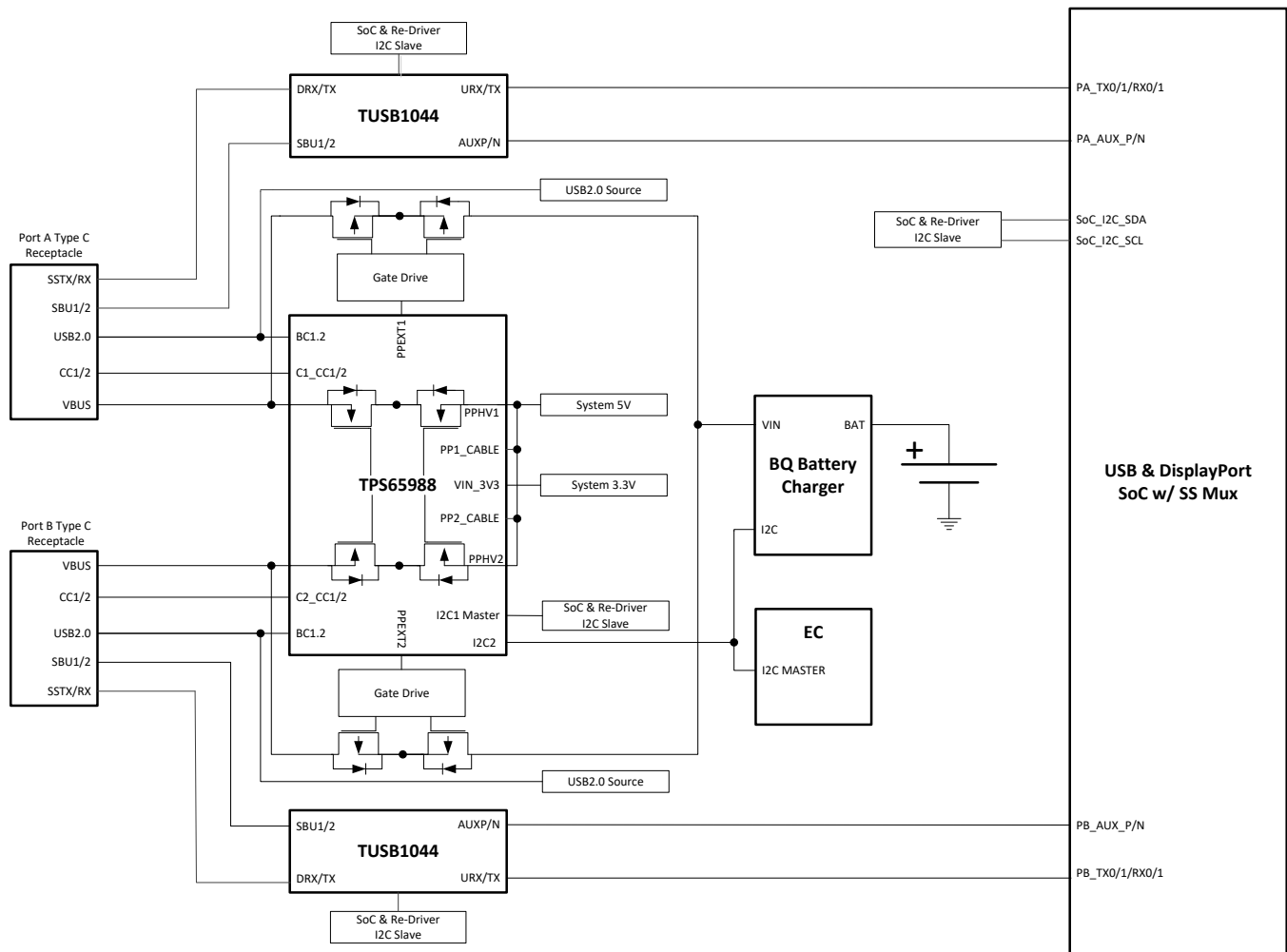
图 43. TPS65988DJ, SoC and Redriver I2C
