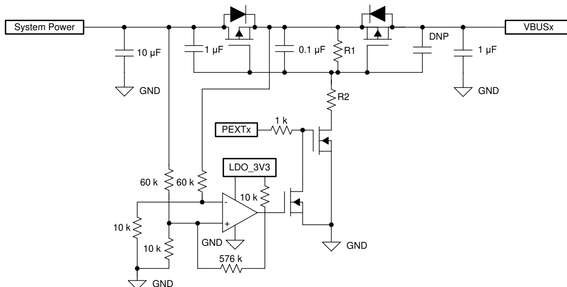
图 34. Recommended Sink Power Path
