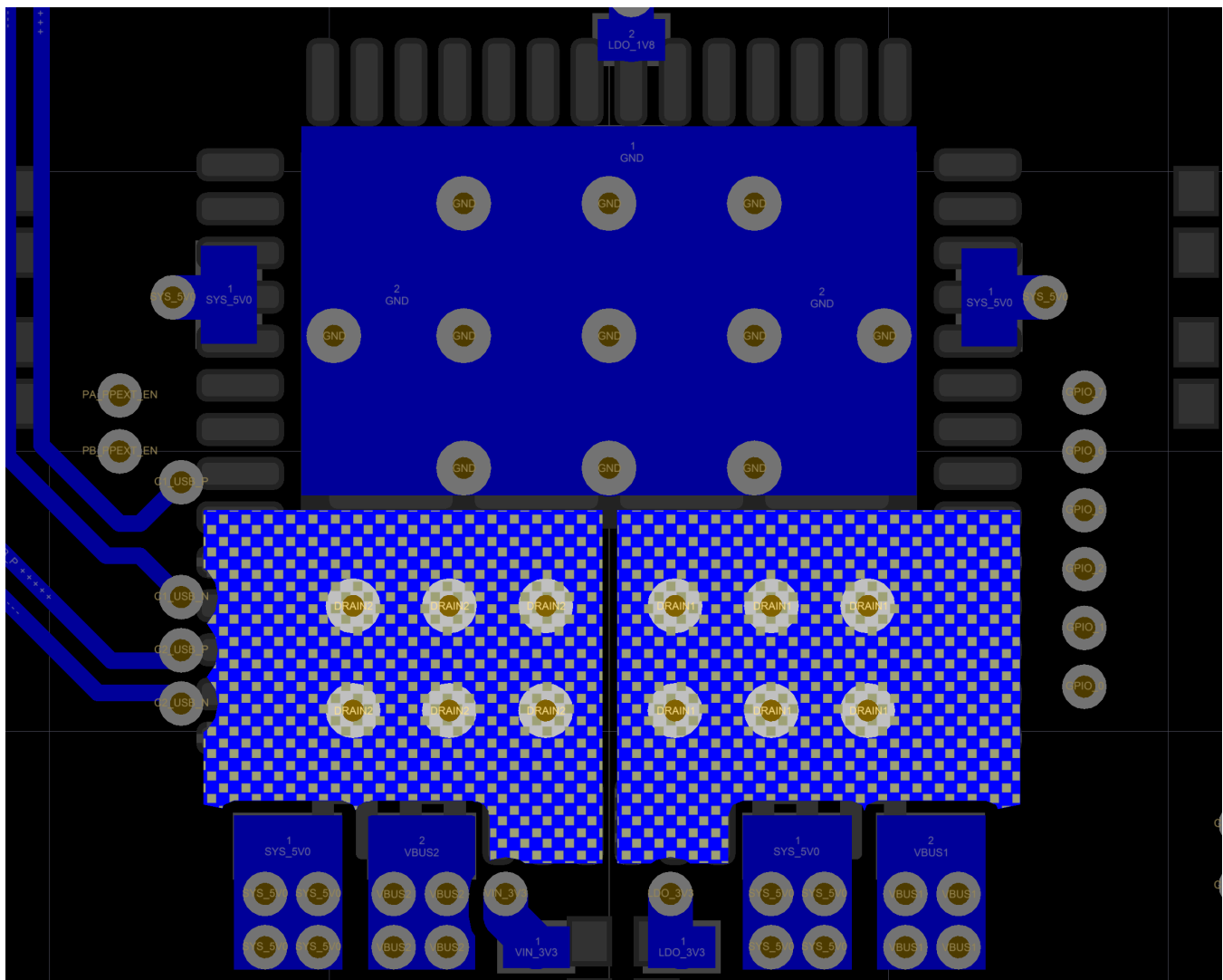
图 60. Figure 13. DRAIN1 and DRAIN2 Bottom Layer
