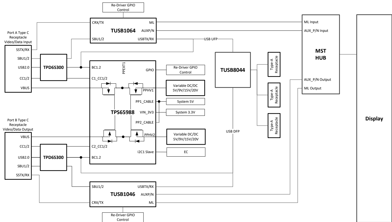
图 44. USB and DisplayPort Dock Block Diagram
