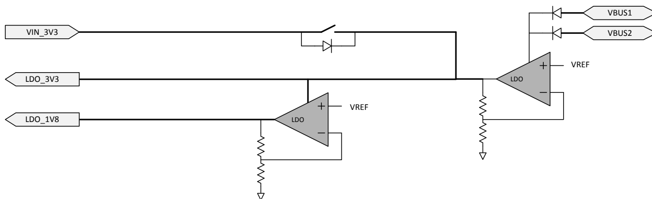
图 13. Power Supplies
