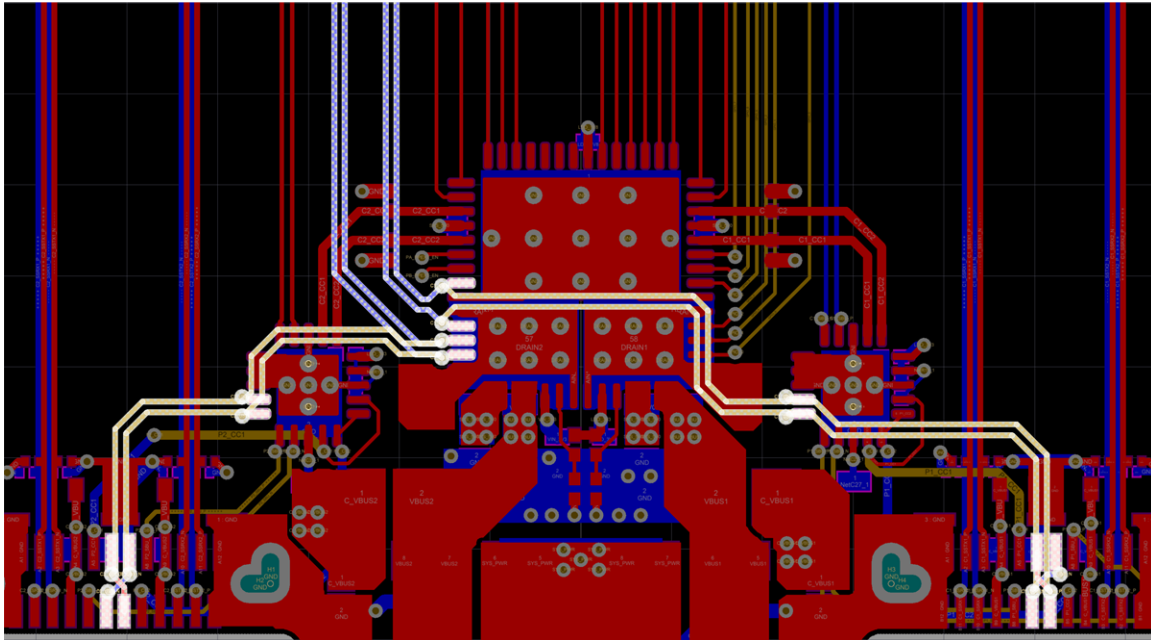
图 61. Complete USB2 Routing
