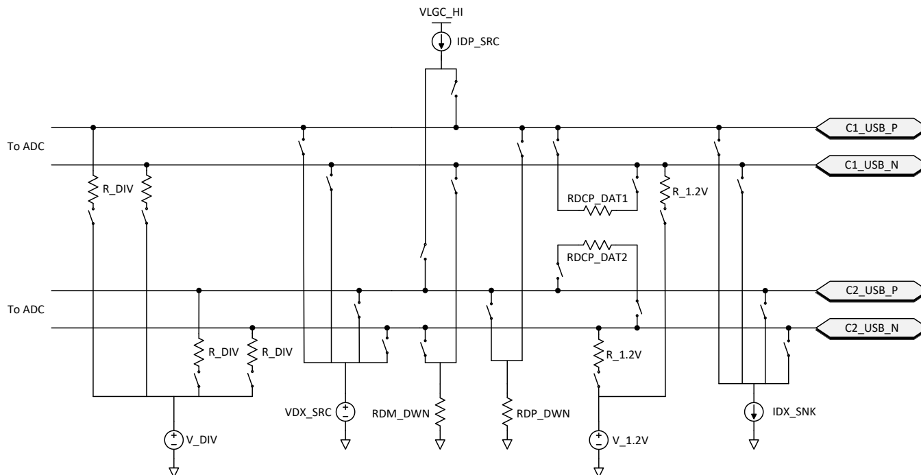
图 22. Battery Charger Detection and Advertisement
