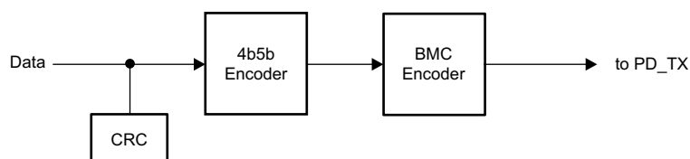
图 6. USB-PD Baseband Transmitter Block Diagram
