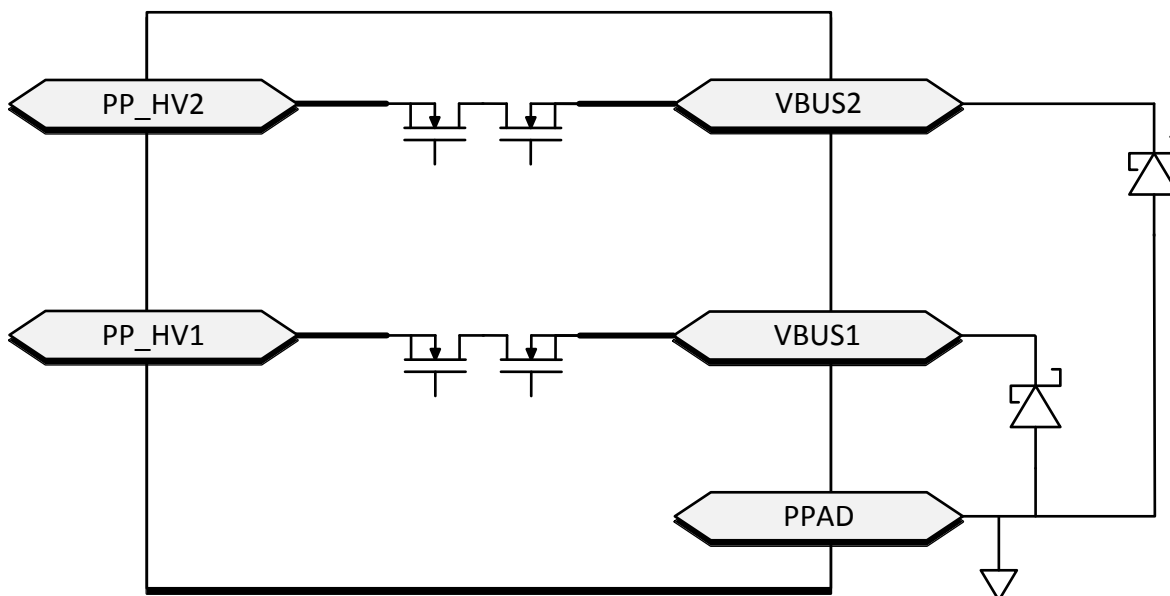
图 17. Schottky for Current Surge Protection
