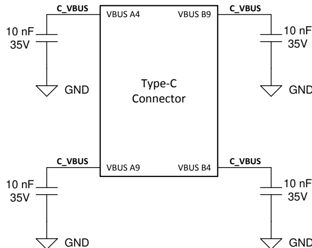
图 36. Type-C Connector VBUS Capacitors
