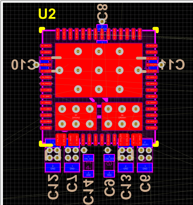
图 53. System Capacitors Placement Top/Bottom Layer
