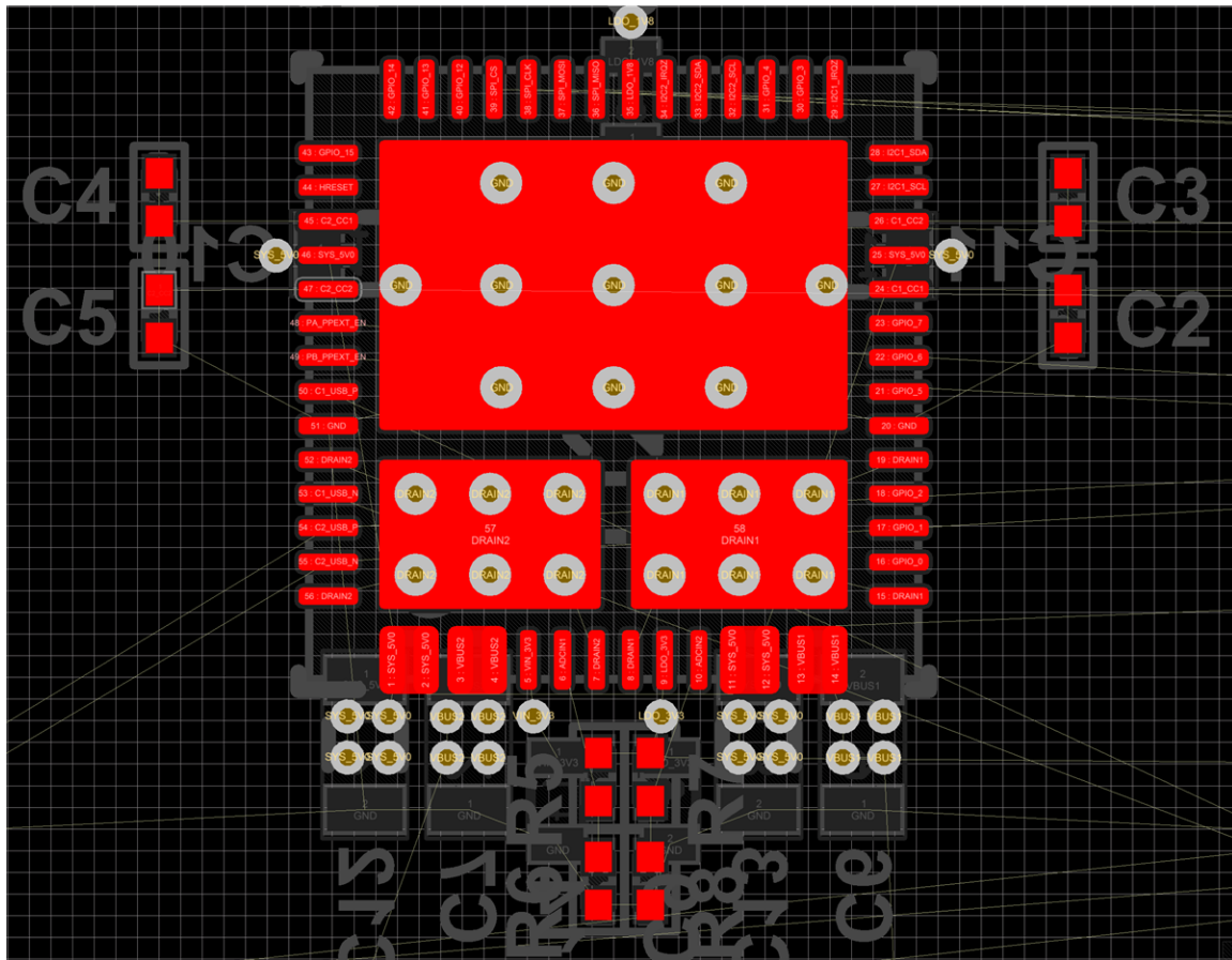
图 56. CC and ADCIN1/2 Component Placements
