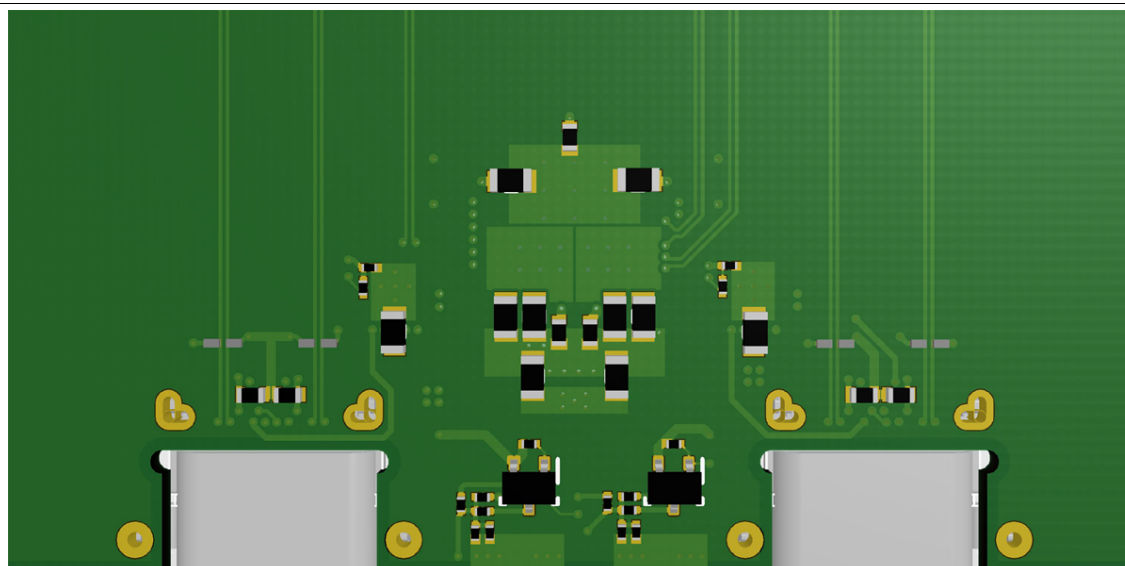
图 72. Bottom 3D View
