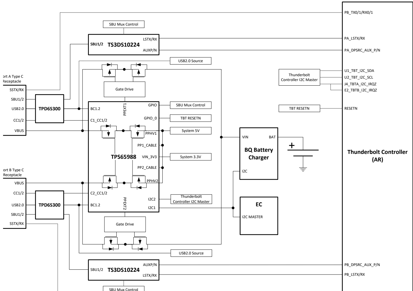
图 40. TBT Notebook with PD Charging
