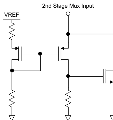
Figure 11. Port Mux Clamp
