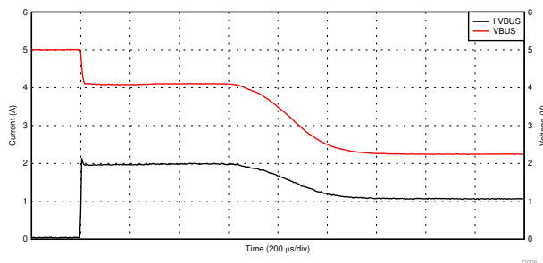
Figure 8. PP_5V0 Current Limit With a Soft Short ( 2\ \Omega )
