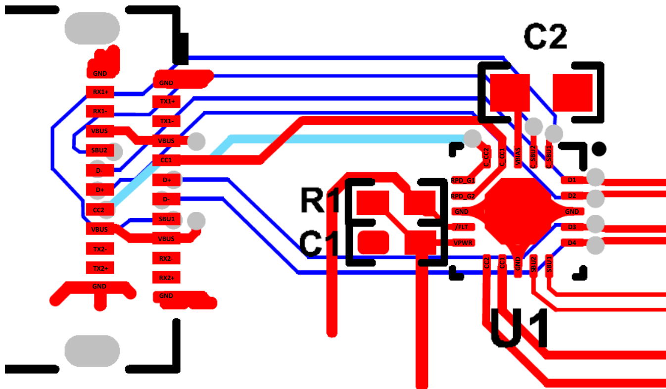
图 34. TPD8S300 Typical Layout
