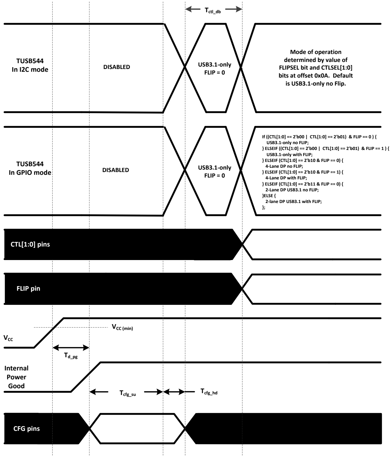
图 21. Power-Up Timing
