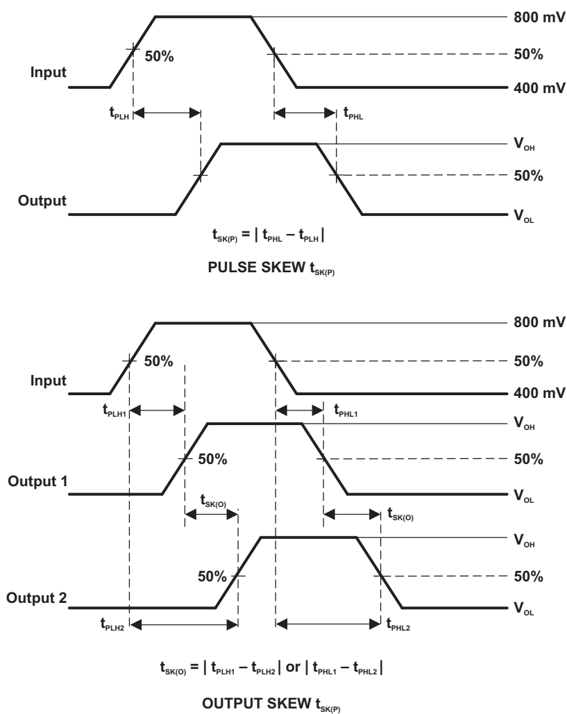
Figure 11. Skew Test
