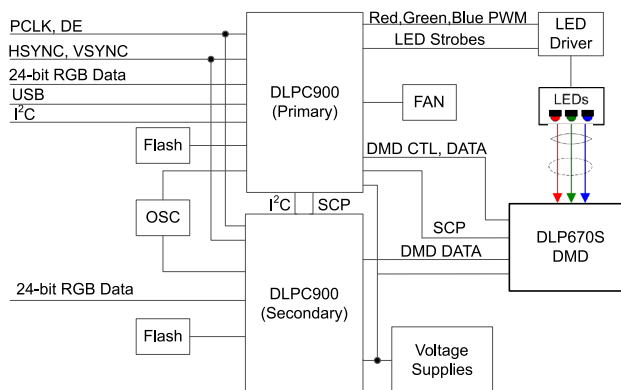
Figure 3-1. DLP670S Simplified Schematic
