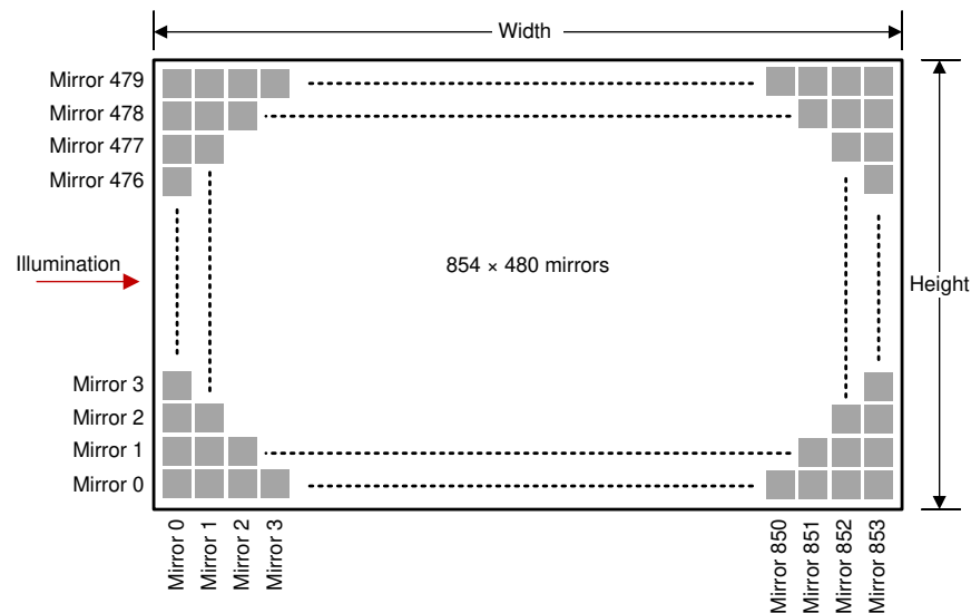
Figure 16. Micromirror Array Physical Characteristics
