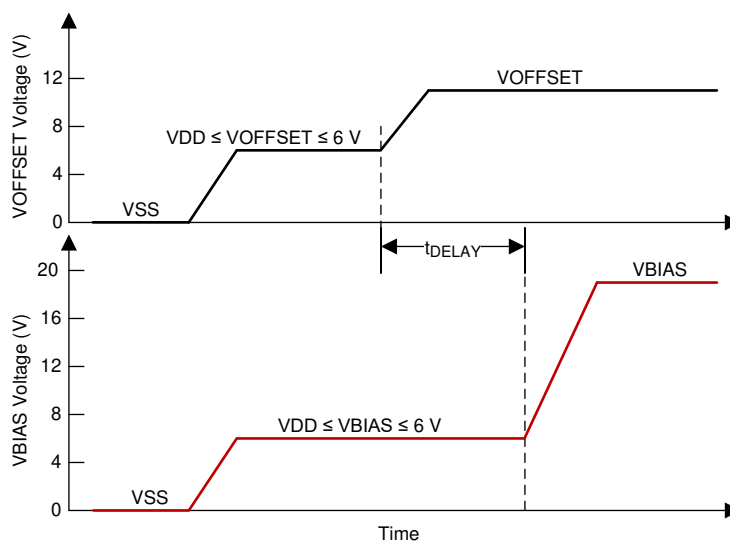
Figure 24. Power-Up Sequence Delay Requirement
