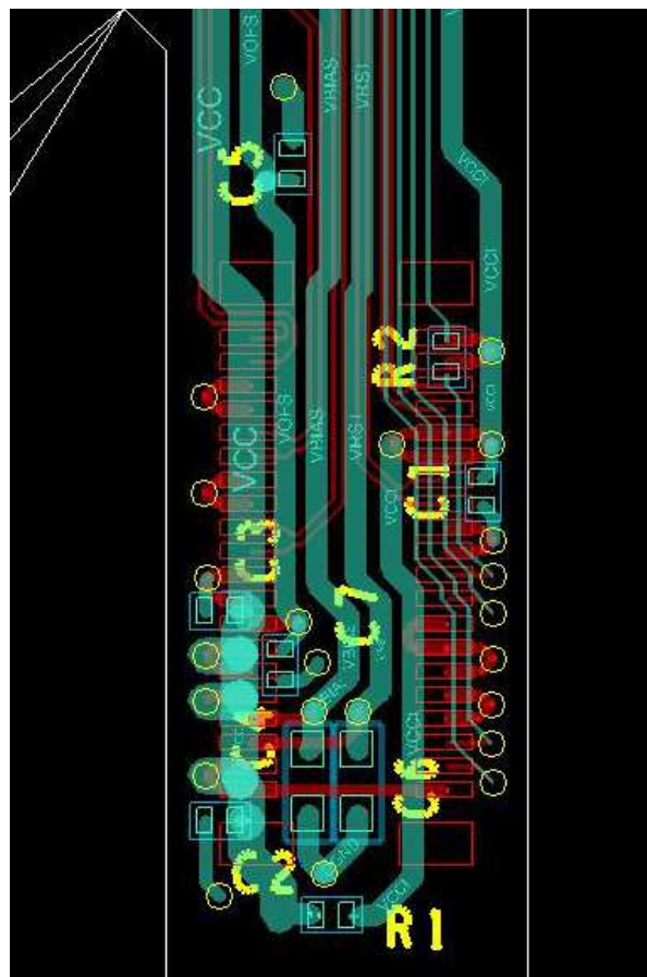
Figure 26. Power Supply Connections
