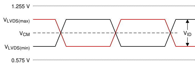
Figure 9. SubLVDS Voltage Parameters
