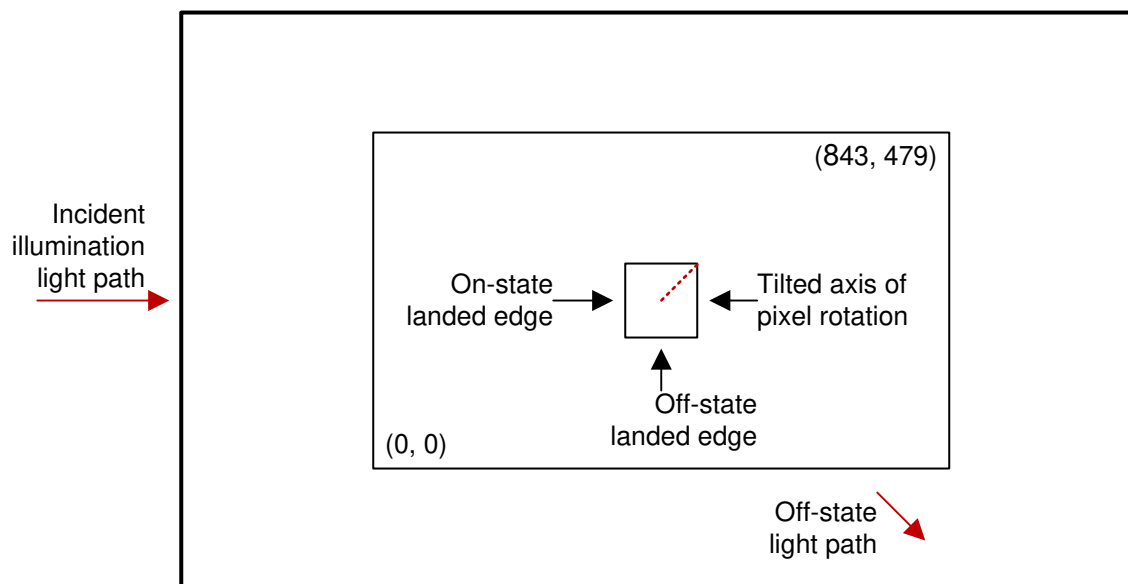
Figure 18. Landed Pixel Orientation and Tilt
