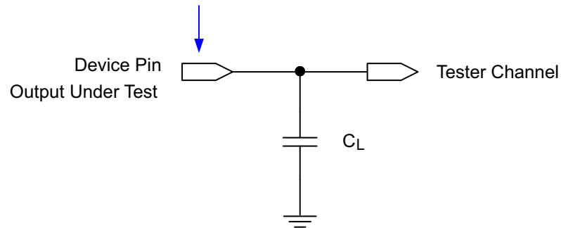
Figure 14. Test Load Circuit for Output Propagation Measurement
