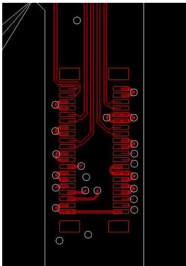
Figure 25. High-Speed (HS) Bus Connections
