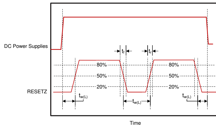
图 6-6. Power-Up and Power-Down RESETZ Timing
