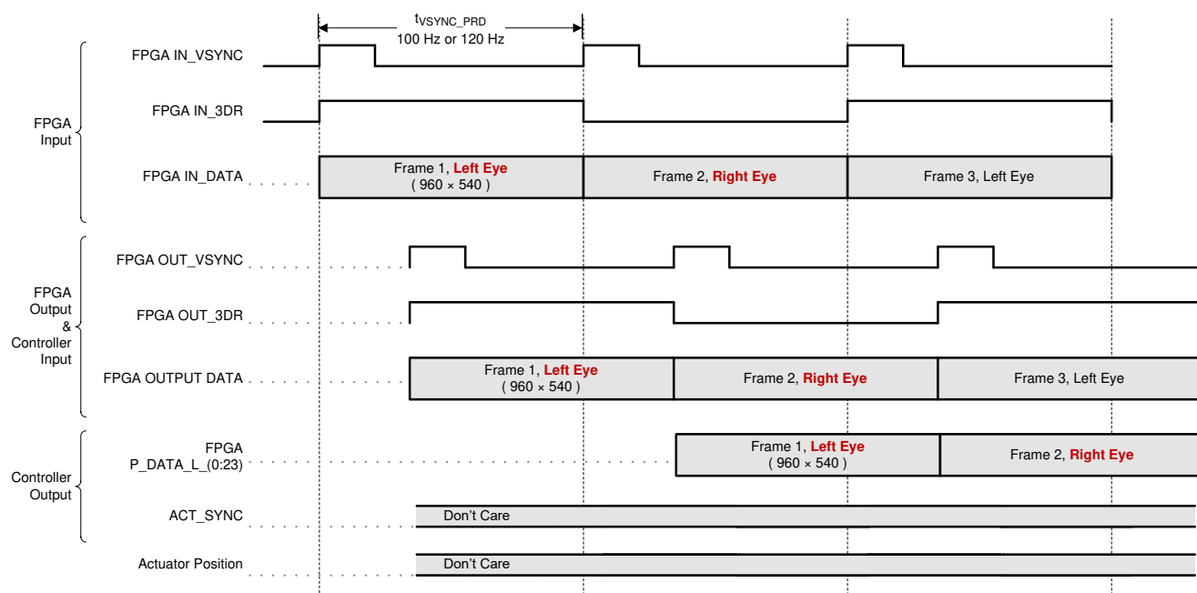
图 7-3. 3D Frame and Signal Timing
