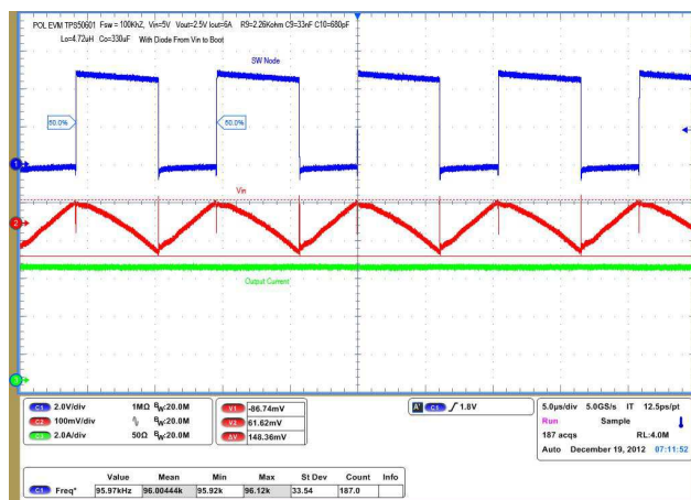
Figure 30. Typical Switching Waveform for 100-kHz Switching Operation
