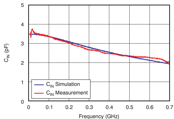
Figure 43. ADC Analog Input Capacitance ( C_{IN} ) Across Frequency
