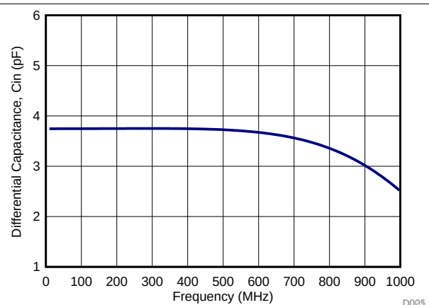
Figure 196. Differential Input Capacitance, C_{IN}
