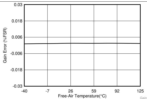
Figure 34. Gain Error in High-Precision Mode vs Temperature
