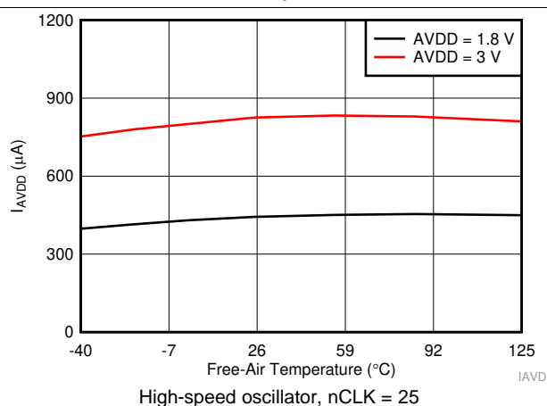
Figure 36. I_{AVDD} in High-Precision Mode vs Temperature
