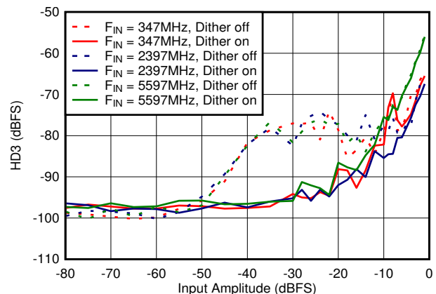
图 6-78. Dual Channel Mode: HD3 vs Input Amplitude and Dither
