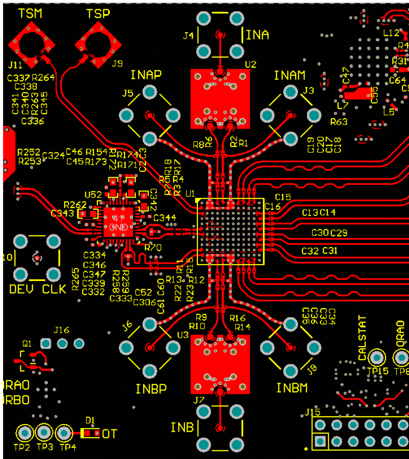
图 10-1. Top Layer Routing: Analog Inputs, CLK and SYSREF, DA0-3, DB0-3
