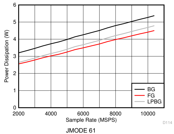
图 6-130. DES Mode: Power Dissipation vs Sample Rate
