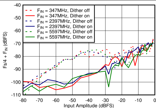
图 6-66. DES Mode: F_s/2 - F_{\text{IN}} vs Input Amplitude and Dither
