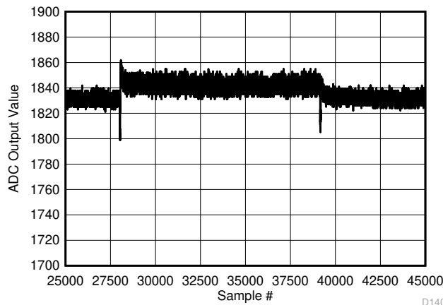
图 6-145. Background Calibration Core Transition (DC Signal - zoomed)
