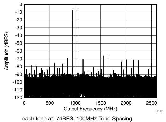
图 6-26. DES Mode: Two Tone FFT at 4197MHz
