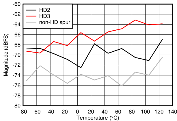
FG calibration at each temperature 图 6-87. DES Mode: HD2, HD3 and Worst non-HD Spur vs Temperature
