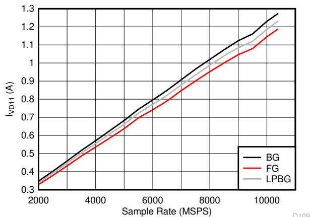
图 6-125. DES Mode: I_{VD11} vs Sample Rate
