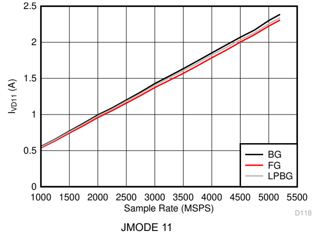
图 6-134. Dual Channel Mode: I_{VD11} vs Sample Rate
