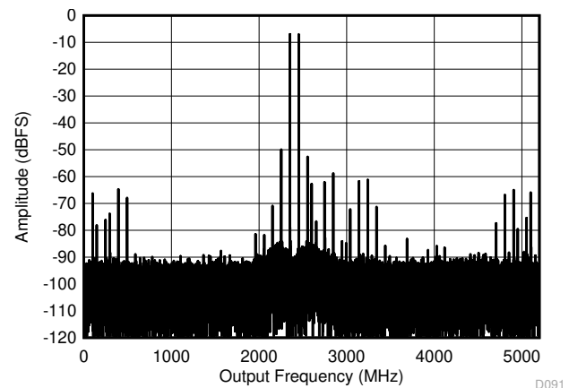
图 6-16. DES Mode: Two Tone FFT at 7997MHz
