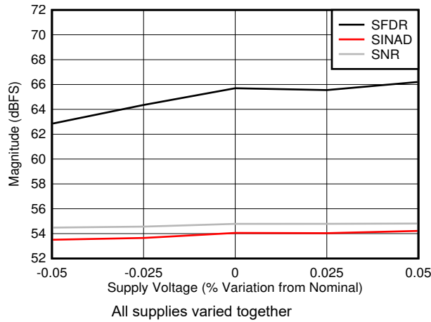
图 6-95. Dual Channel Mode: SNR, SINAD and SFDR vs Supply Voltage
