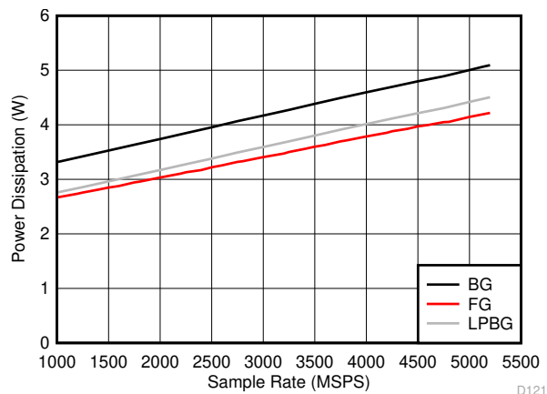
图 6-137. Dual Channel Mode: Power Dissipation vs Sample Rate
