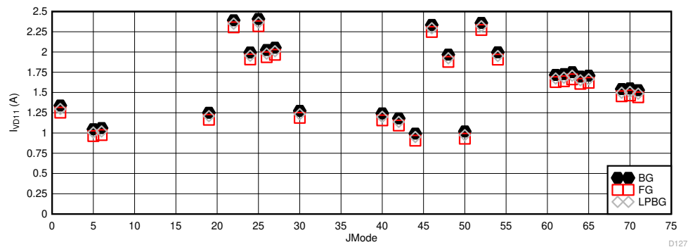
图 6-110. DES Mode: I_{VA11} vs JMODE at 10.4GSPS
