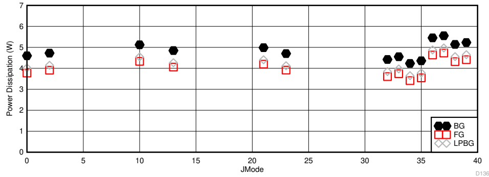
图 6-119. Other Modes with Lower Maximum F_S : I_{VD11} vs JMODE
