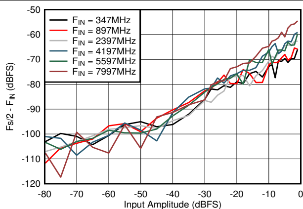
图 6-65. DES Mode: F_s/2 - F_{\text{IN}} vs Input Amplitude and Frequency
