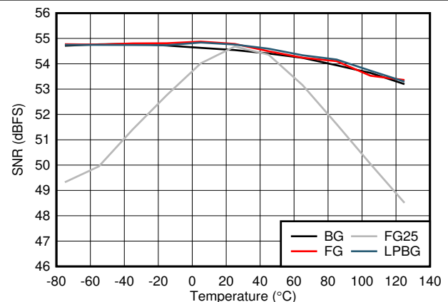
FG25 is calibrated at 25^\circ\text{C} and held at other temperatures, other modes recalibrated at each temperature 图 6-90. Dual Channel Mode: SNR vs Temperature and Calibration Mode
