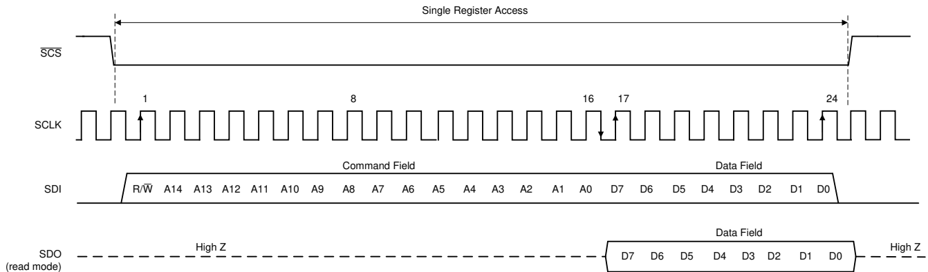
图 7-27. Serial Interface Protocol: Single Read/Write
