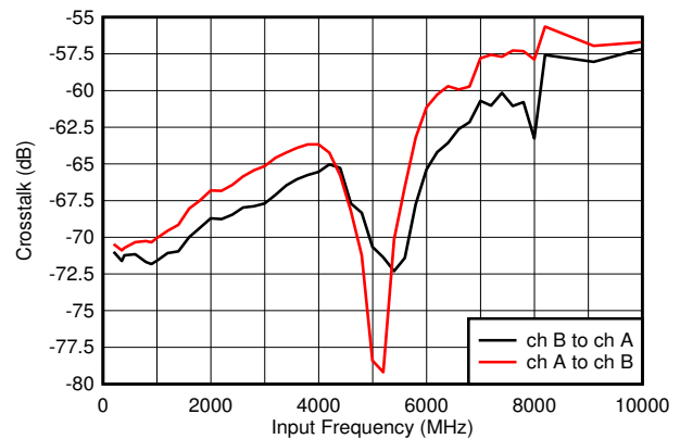
Dual channel mode, JMODE 3 图 6-2. Crosstalk vs Input Frequency
