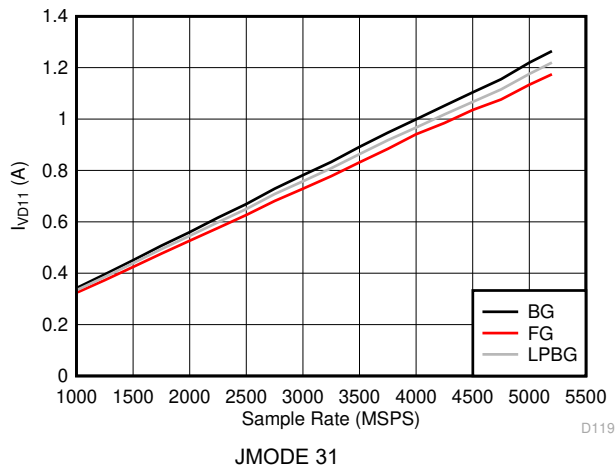
图 6-135. Dual Channel Mode: I_{VD11} vs Sample Rate
