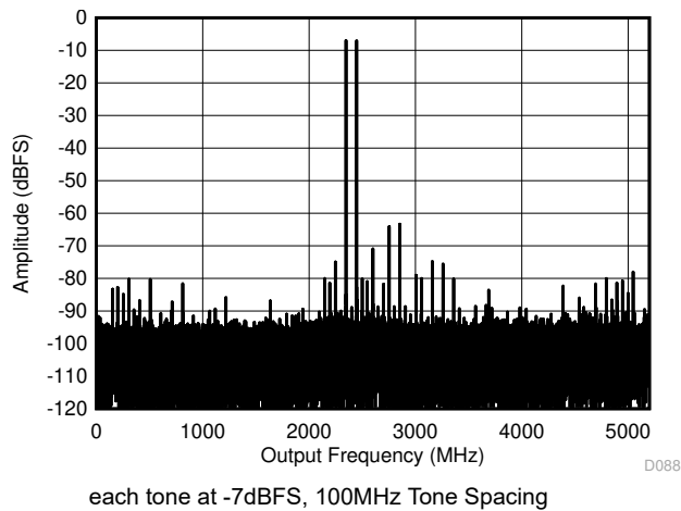
图 6-13. DES Mode: Two Tone FFT at 2397MHz
