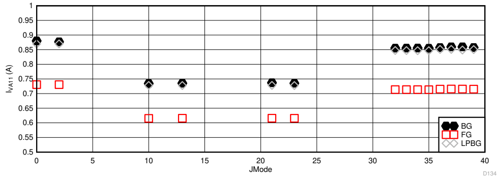
图 6-118. Other Modes with Lower Maximum F_S : I_{VA11} vs JMODE
