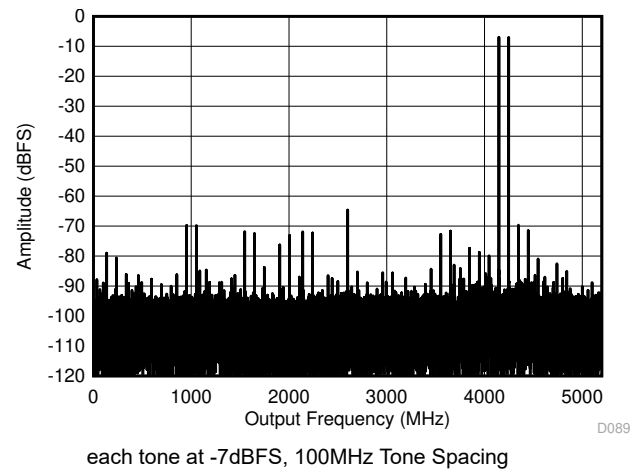
图 6-14. DES Mode: Two Tone FFT at 4197MHz
