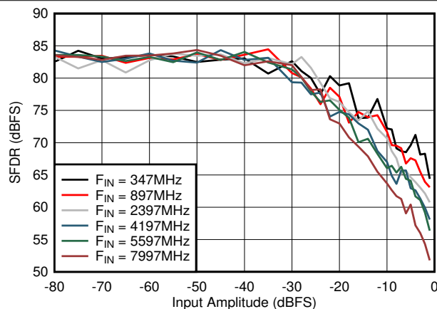
图 6-59. DES Mode: SFDR vs Input Amplitude and Frequency
