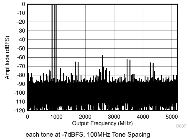
图 6-12. DES Mode: Two Tone FFT at 897MHz
