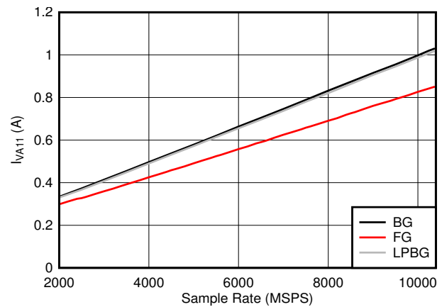
图 6-122. DES Mode: I_{VA11} vs Sample Rate
