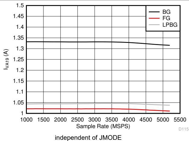
图 6-131. Dual Channel Mode: I_{VA19} vs Sample Rate
