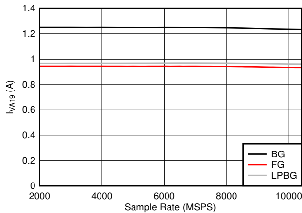
图 6-121. DES Mode: I_{VA19} vs Sample Rate
