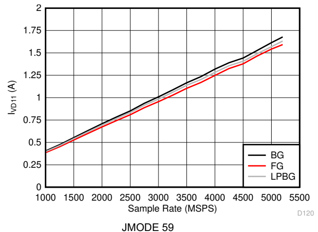
图 6-136. Dual Channel Mode: I_{VD11} vs Sample Rate
