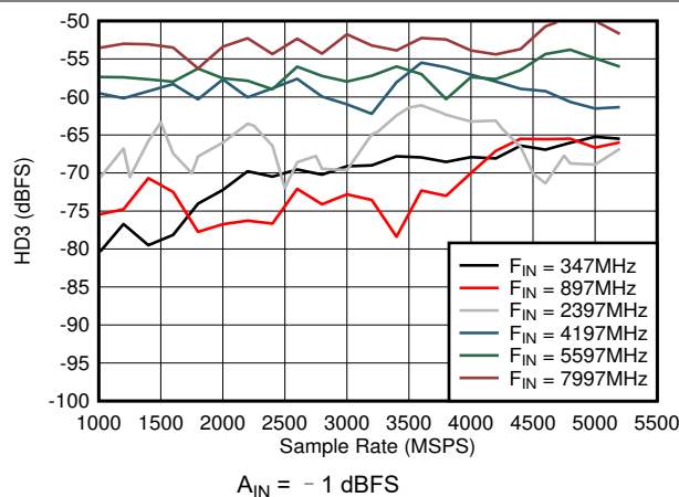
图 6-53. Dual Channel Mode: HD3 vs Sample Rate and Input Frequency
