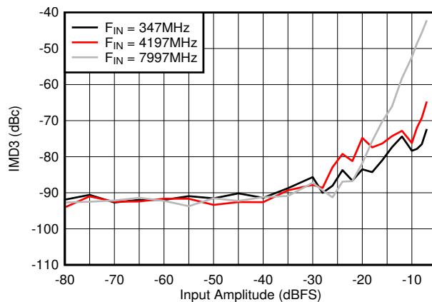
图 6-105. Dual Channel Mode: IMD3 vs Input Amplitude
