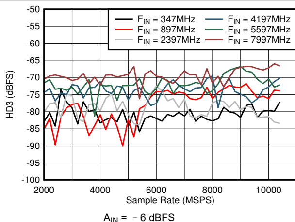
图 6-39. DES Mode: HD3 vs Sample Rate and Input Frequency
