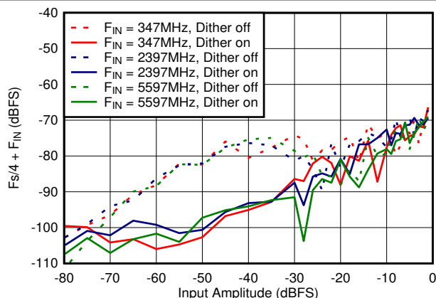
图 6-68. DES Mode: F_s/4 + F_{\text{IN}} vs Input Amplitude and Dither
