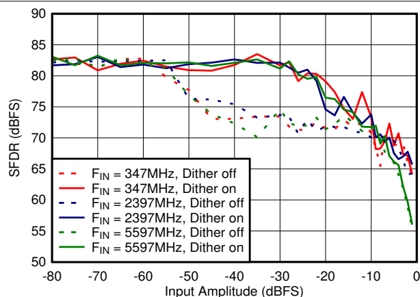
图 6-74. Dual Channel Mode: SFDR vs Input Amplitude and Dither
