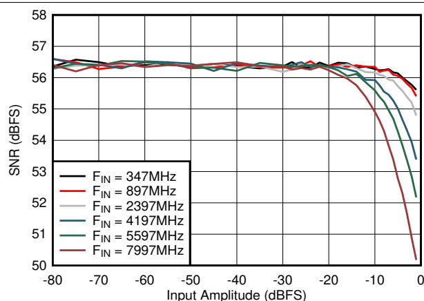
图 6-71. Dual Channel Mode: SNR vs Input Amplitude and Frequency
