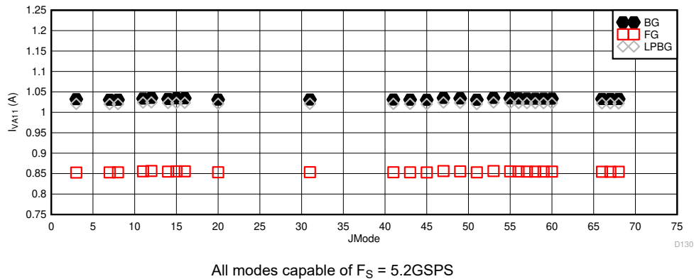
图 6-114. Dual Channel Mode: I_{V_{A11}} vs JMODE at 5.2GSPS
