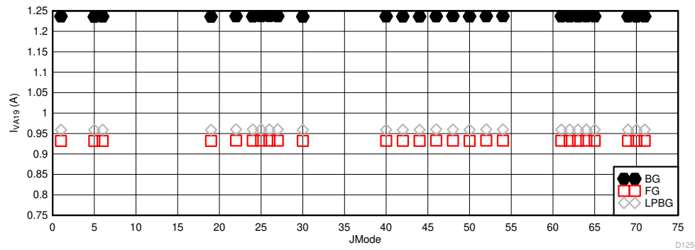
图 6-109. DES Mode: I_{VA19} vs JMODE at 10.4GSPS
