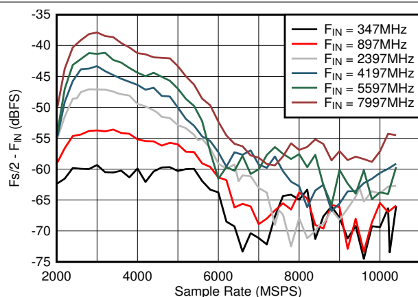
图 6-41. DES Mode: F_s/2 - F_{\text{IN}} vs Sample Rate and Input Frequency
