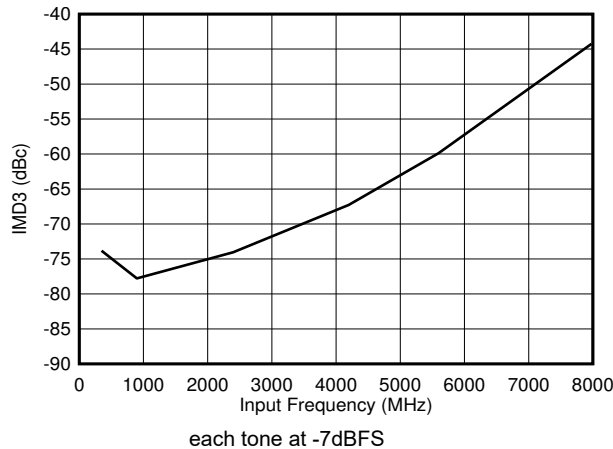
图 6-99. DES Mode: IMD3 vs Input Frequency
