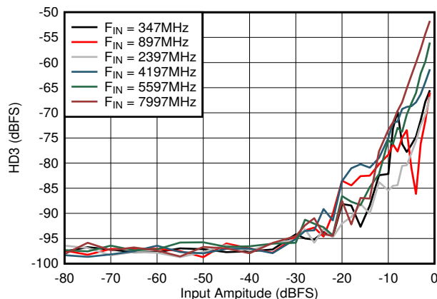
图 6-77. Dual Channel Mode: HD3 vs Input Amplitude and Frequency
