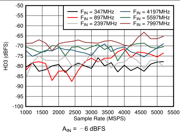
图 6-54. Dual Channel Mode: HD3 vs Sample Rate and Input Frequency
