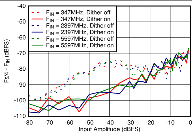
图 6-70. DES Mode: F_s/4 - F_{\text{IN}} vs Input Amplitude and Dither
