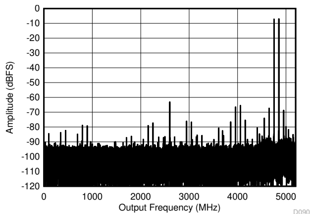
图 6-15. DES Mode: Two Tone FFT at 5597MHz
