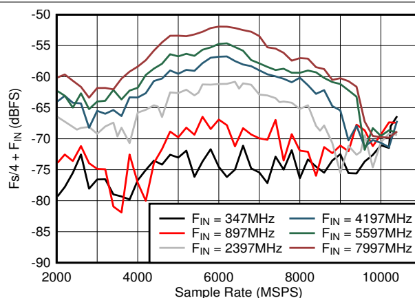
图 6-42. DES Mode: F_s/4 + F_{\text{IN}} vs Sample Rate and Input Frequency
