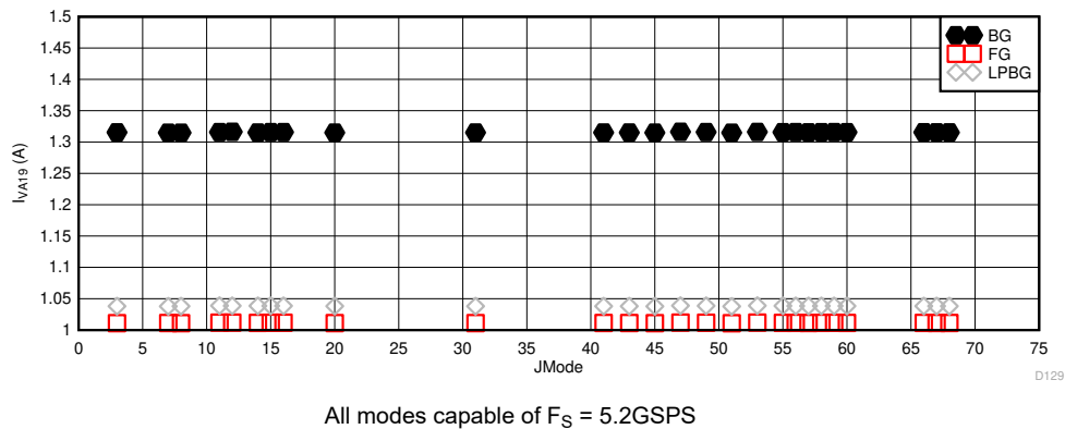
图 6-113. Dual Channel Mode: I_{V_{A19}} vs JMODE at 5.2GSPS
