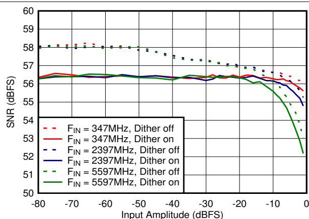
图 6-72. Dual Channel Mode: SNR vs Input Amplitude and Dither
