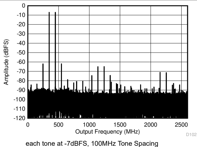
图 6-27. DES Mode: Two Tone FFT at 5597MHz
