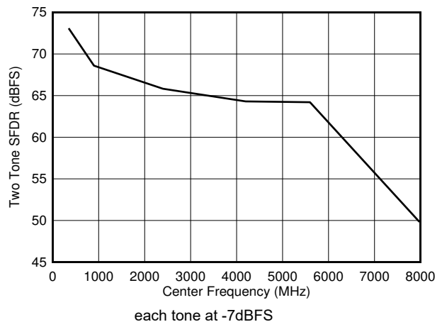
图 6-102. DES Mode: Two Tone SFDR vs Input Frequency
