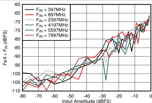
图 6-67. DES Mode: F_s/4 + F_{\text{IN}} vs Input Amplitude and Frequency
