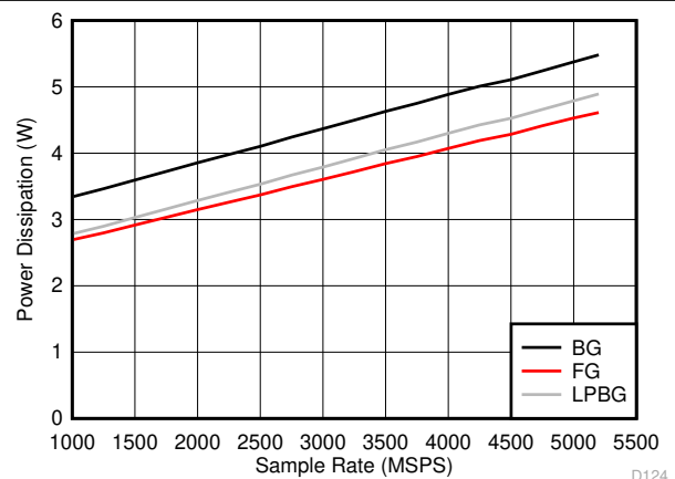
图 6-138. Dual Channel Mode: Power Dissipation vs Sample Rate
