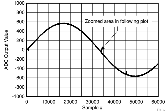
图 6-142. Background Calibration Core Transition (AC Signal)
