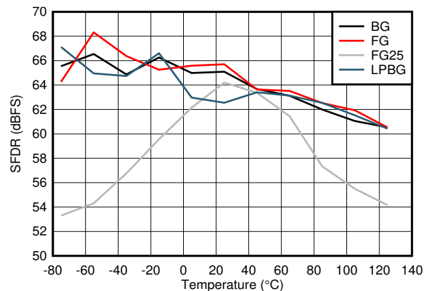
图 6-92. Dual Channel Mode: SFDR vs Temperature and Calibration Mode
