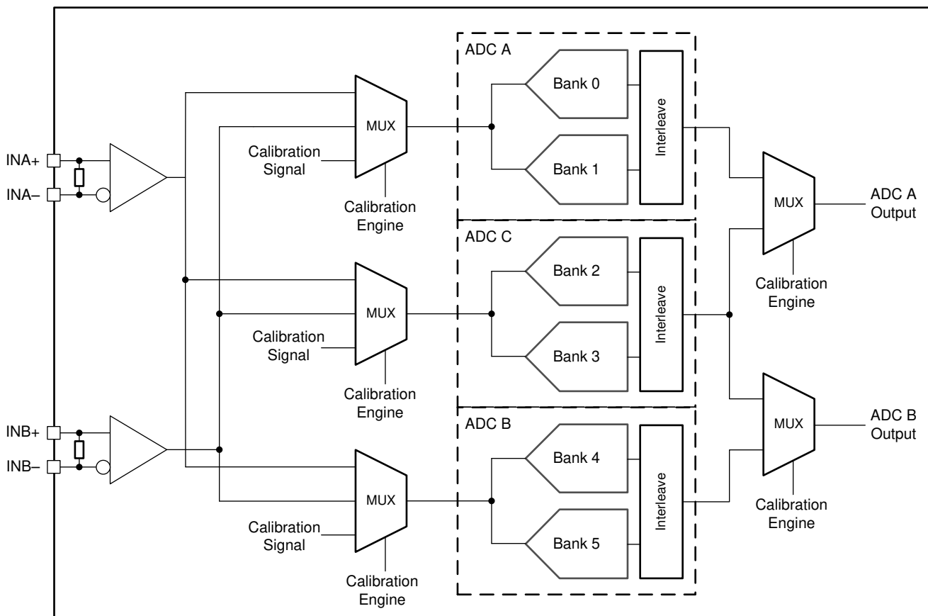
图 7-26. ADC12DJ5200RF Calibration System Block Diagram
