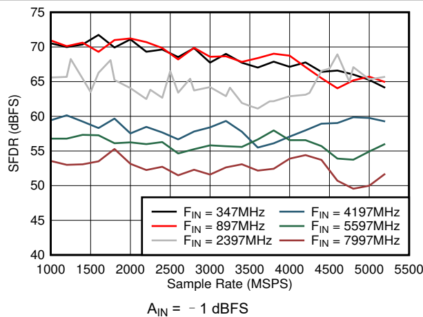
图 6-47. Dual Channel Mode: SFDR vs Sample Rate and Input Frequency
