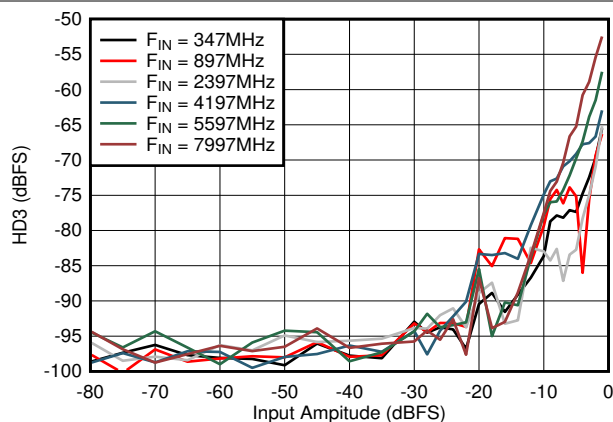
图 6-63. DES Mode: HD3 vs Input Amplitude and Frequency
