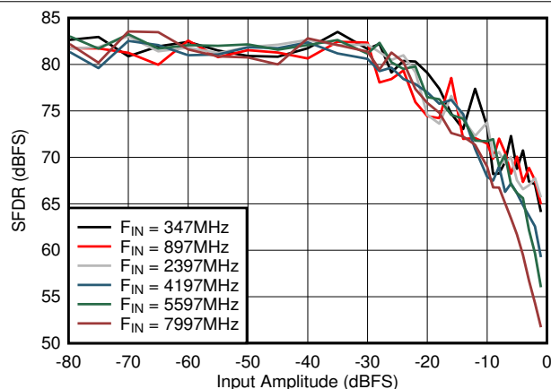
图 6-73. Dual Channel Mode: SFDR vs Input Amplitude and Frequency
