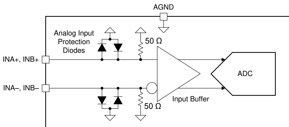
图 7-1. ADC12DJ5200RF Analog Input Internal Termination and Protection Diagram
