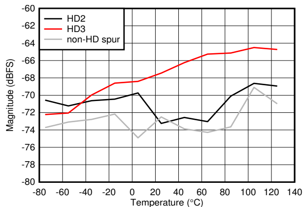
图 6-91. Dual Channel Mode: HD2, HD3 and Worst non-HD Spur vs Temperature
