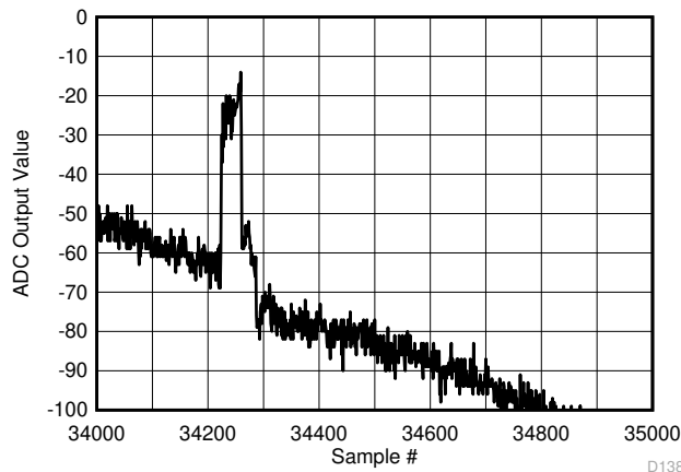
图 6-143. Background Calibration Core Transition (AC Signal - zoomed)
