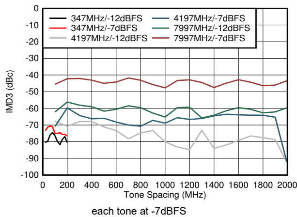
图 6-101. DES Mode: IMD3 vs Tone Spacing
