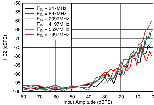
图 6-75. Dual Channel Mode: HD2 vs Input Amplitude and Frequency
