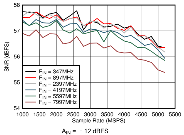
图 6-46. Dual Channel Mode: SNR vs Sample Rate and Input Frequency
