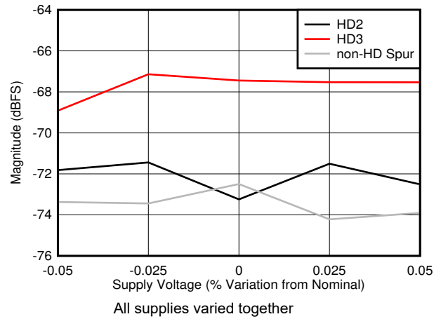
图 6-96. Dual Channel Mode: HD2, HD3 and Worst non-HD Spur vs Supply Voltage
