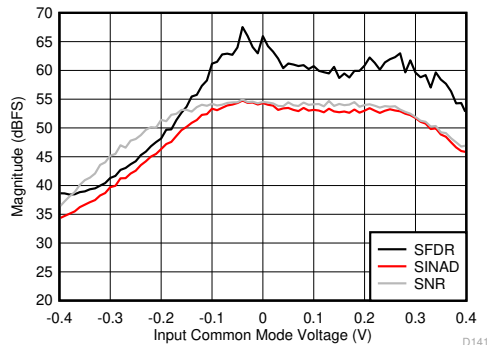
图 6-97. SNR, SFDR and SINAD vs Input Common Mode Voltage
