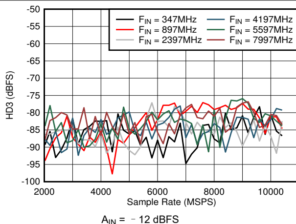
图 6-40. DES Mode: HD3 vs Sample Rate and Input Frequency
