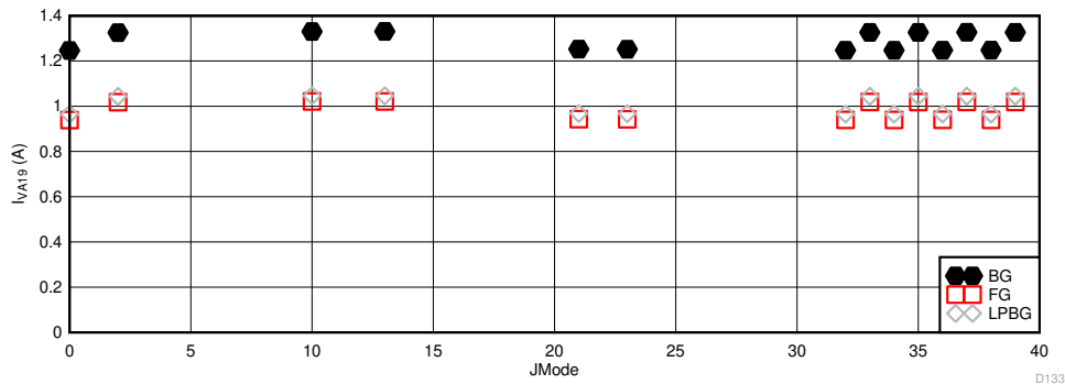
图 6-116. Dual Channel Mode: Power Dissipation vs JMODE at 5.2GSPS
