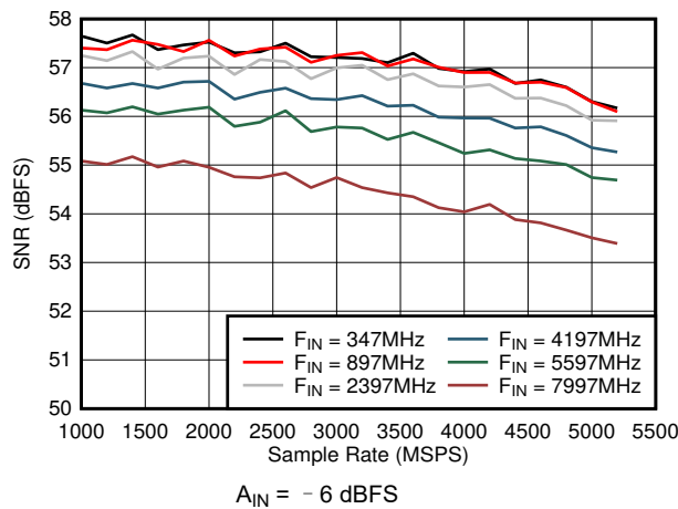
图 6-45. Dual Channel Mode: SNR vs Sample Rate and Input Frequency
