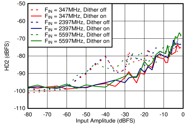
图 6-76. Dual Channel Mode: HD2 vs Input Amplitude and Dither
