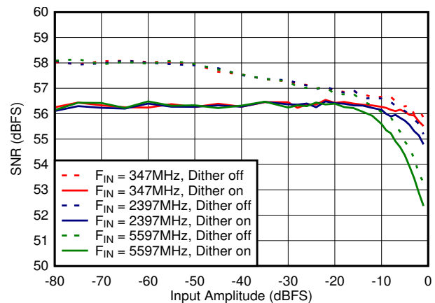
图 6-58. DES Mode: SNR vs Input Amplitude and Dither
