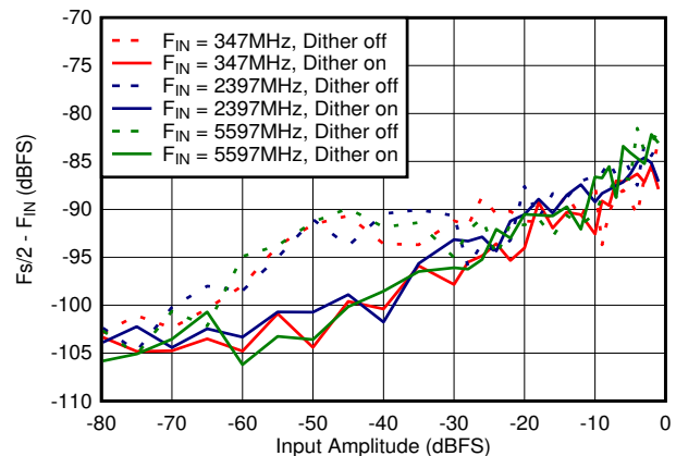
图 6-80. Dual Channel Mode: F_s/2 - F_{\text{IN}} vs Input Amplitude and Dither
