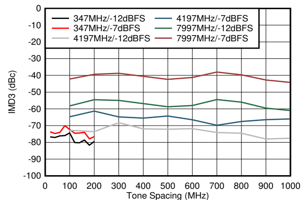
图 6-106. Dual Channel Mode: IMD3 vs Tone Spacing
