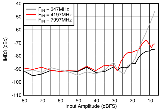
图 6-100. DES Mode: IMD3 vs Input Amplitude
