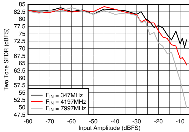
图 6-103. DES Mode: Two Tone SFDR vs Input Amplitude
