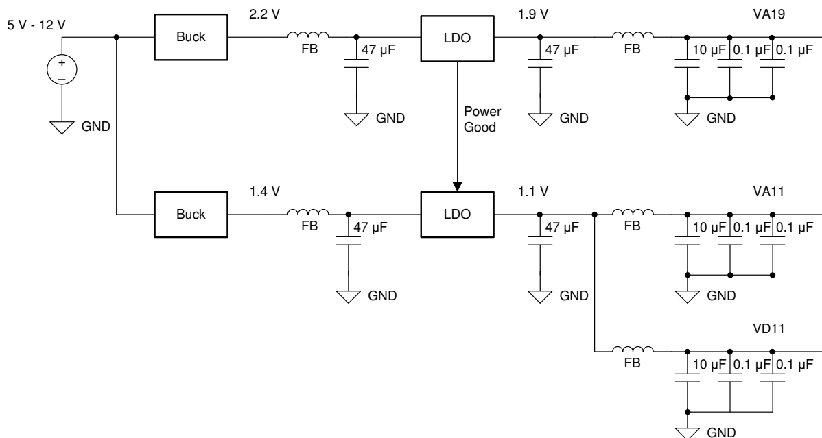
图 9-1. LDO Linear Regulator Approach Example
