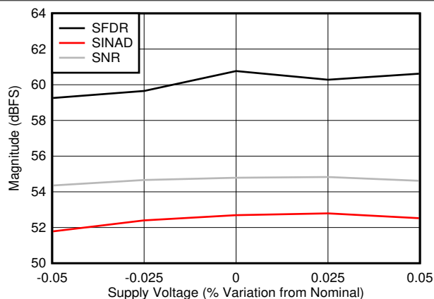
图 6-93. DES Mode: SNR, SINAD and SFDR vs Supply Voltage
