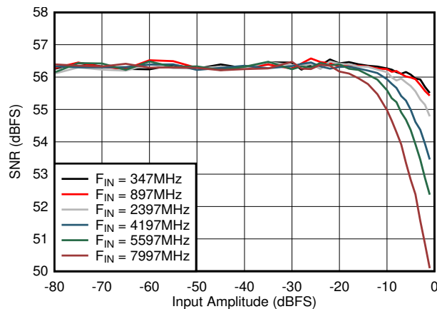
图 6-57. DES Mode: SNR vs Input Amplitude and Frequency
