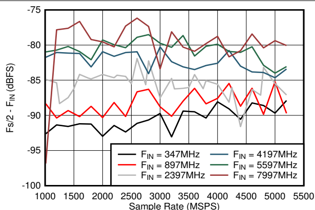
图 6-56. Dual Channel Mode: F_s/2 - F_{\text{IN}} vs Sample Rate and Input Frequency
