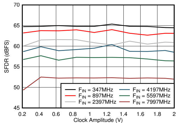
图 6-82. DES Mode: SFDR vs Clock Amplitude
