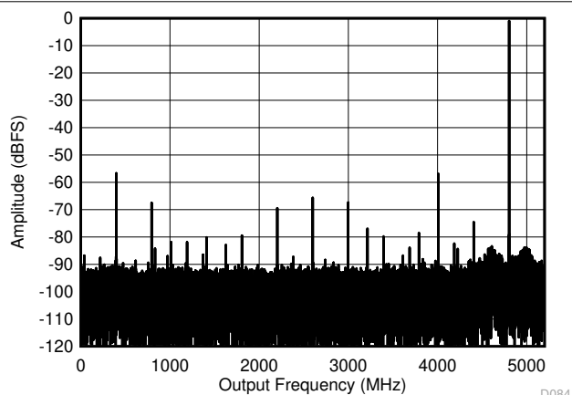
图 6-9. DES Mode: Single Tone FFT at 5597MHz
