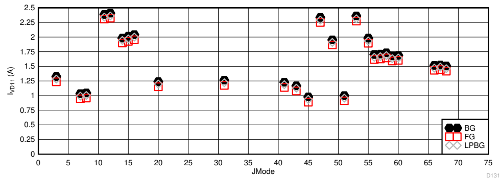
图 6-115. Dual Channel Mode: I_{VD11} vs JMODE at 5.2GSPS
