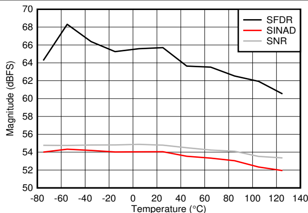
FG calibration at each temperature 图 6-89. Dual Channel Mode: SNR, SINAD and SFDR vs Temperature
