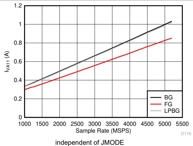
图 6-132. Dual Channel Mode: I_{VA11} vs Sample Rate
