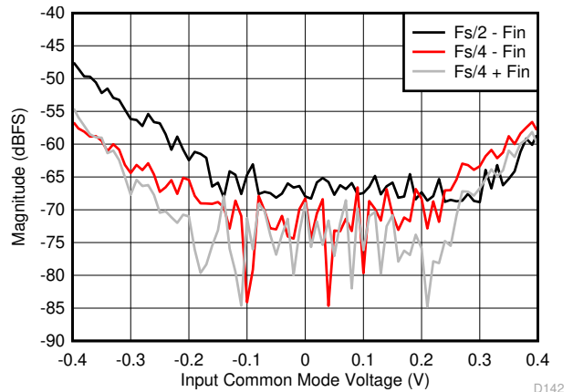
图 6-98. F_s/2 - F_{\text{IN}} and F_s/4 \pm F_{\text{IN}} vs Input Common Mode Voltage
