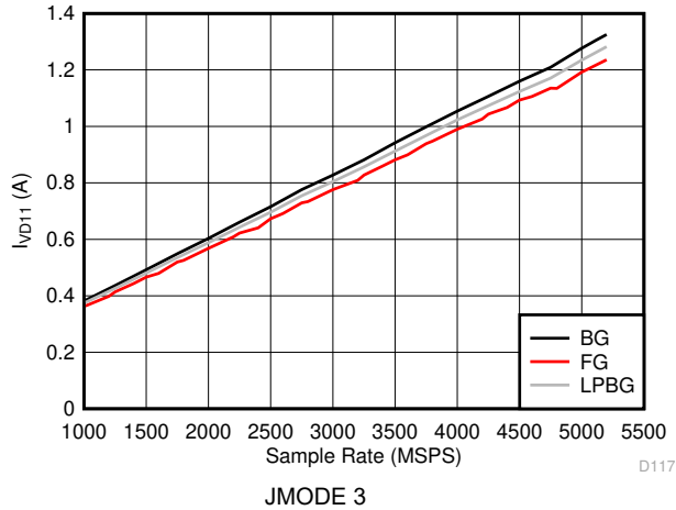
图 6-133. Dual Channel Mode: I_{VD11} vs Sample Rate
