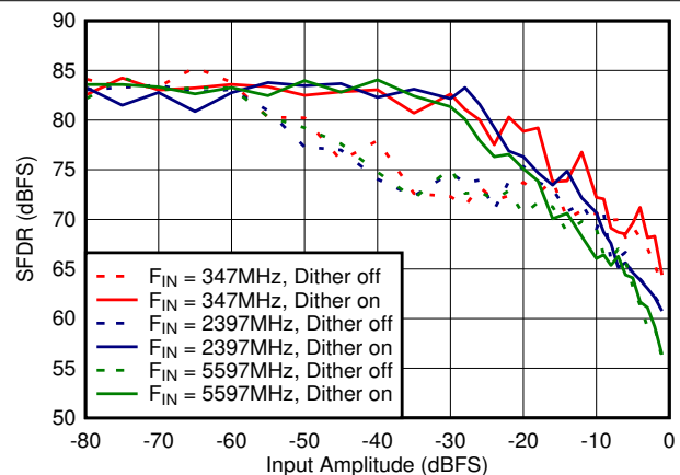
图 6-60. DES Mode: SFDR vs Input Amplitude and Dither
