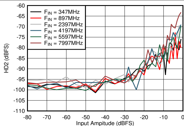
图 6-61. DES Mode: HD2 vs Input Amplitude and Frequency
