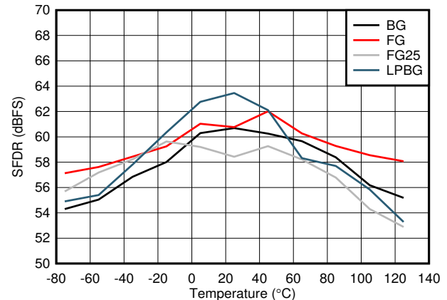
FG25 is calibrated at 25^\circ\text{C} and held at other temperatures, other modes recalibrated at each temperature 图 6-88. DES Mode: SFDR vs Temperature and Calibration Mode
