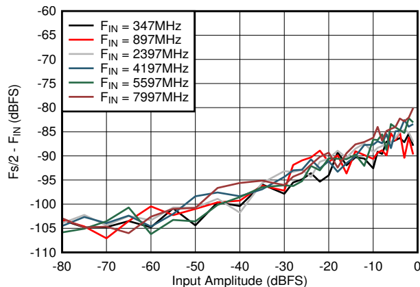
图 6-79. Dual Channel Mode: F_s/2 - F_{\text{IN}} vs Input Amplitude and Frequency
