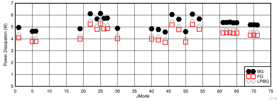
图 6-112. DES Mode: Power Dissipation vs JMODE at 10.4GSPS
