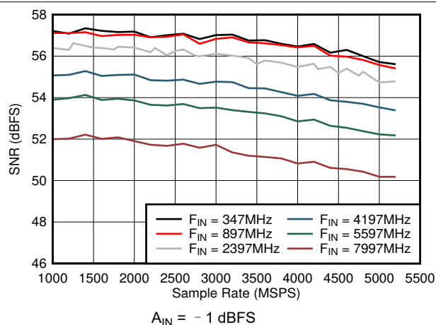
图 6-44. Dual Channel Mode: SNR vs Sample Rate and Input Frequency A_{\text{IN}} = -1\text{ dBFS}
