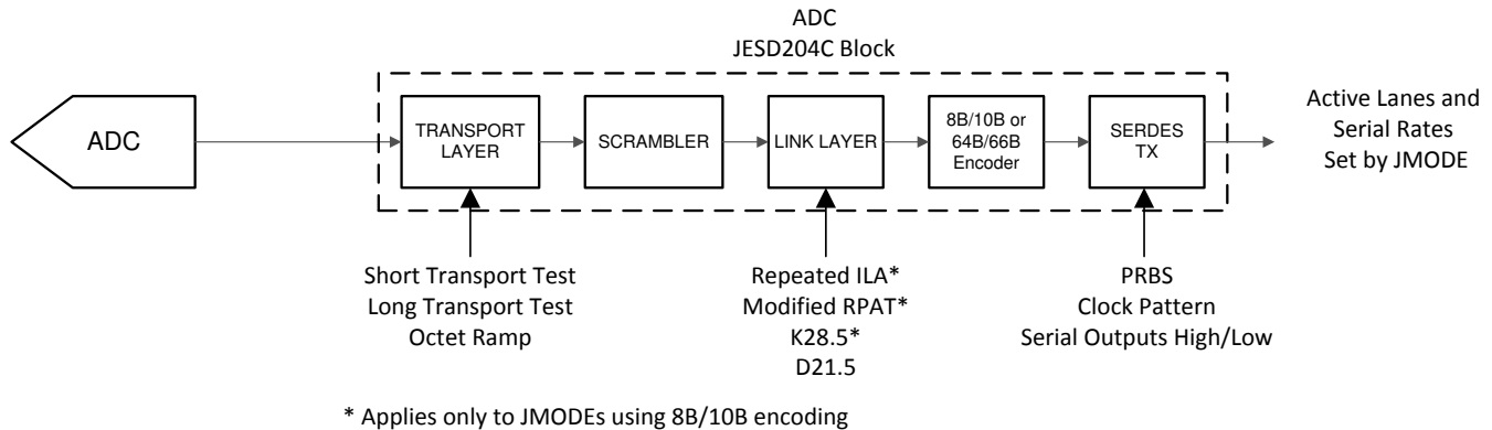
图 7-25. Test Mode Insertion Points
