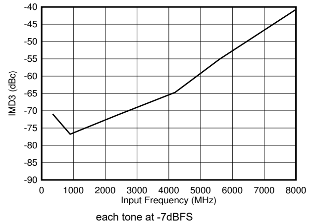
图 6-104. Dual Channel Mode: IMD3 vs Input Frequency
