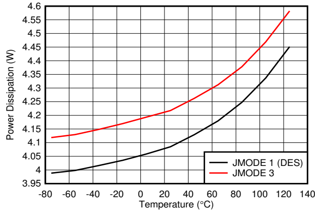
图 6-141. Power Dissipation vs Temperature
