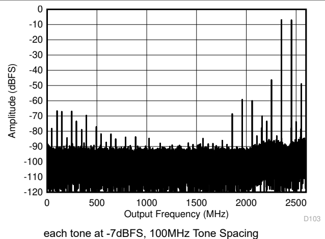
图 6-28. DES Mode: Two Tone FFT at 7997MHz
