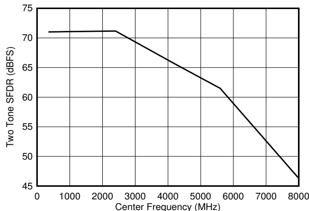
图 6-107. Dual Channel Mode: Two Tone SFDR vs Input Frequency
