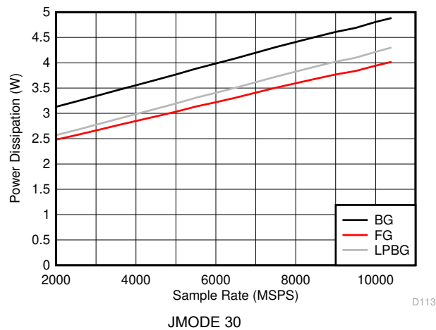
图 6-129. DES Mode: Power Dissipation vs Sample Rate
