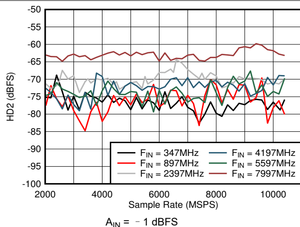
图 6-35. DES Mode: HD2 vs Sample Rate and Input Frequency
