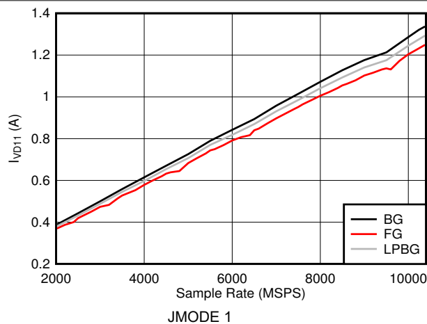
图 6-123. DES Mode: I_{VD11} vs Sample Rate
