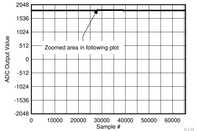
图 6-144. Background Calibration Core Transition (DC Signal)
