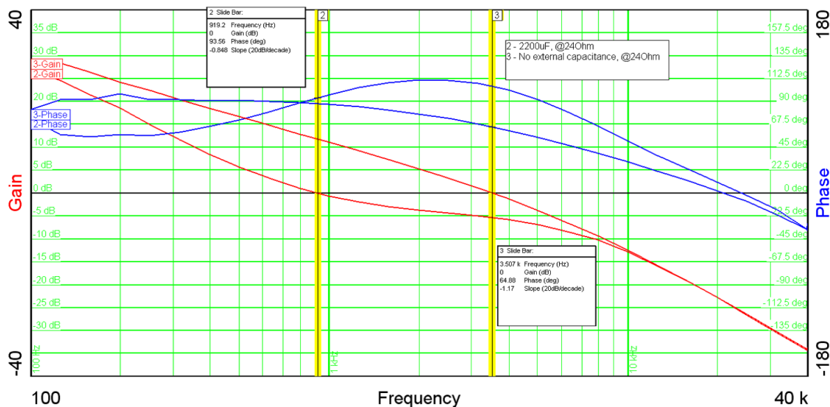
Figure 25. Loop Response
