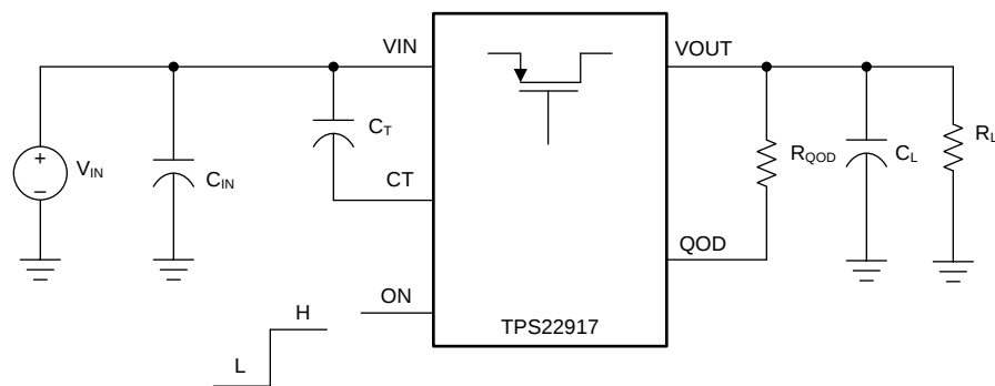
图 33. Typical Application Schematic
