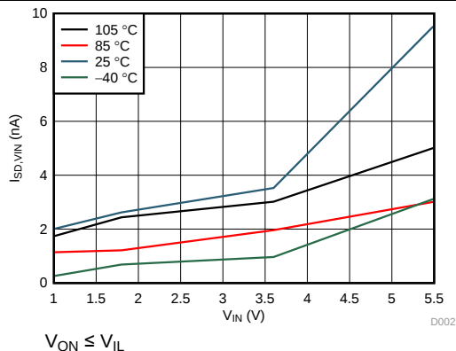
图 1. Shutdown Current ( I_{SD} )
