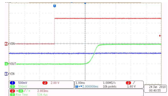
图 16. Turn On at 3.6 V (CT = 1000 pF)
