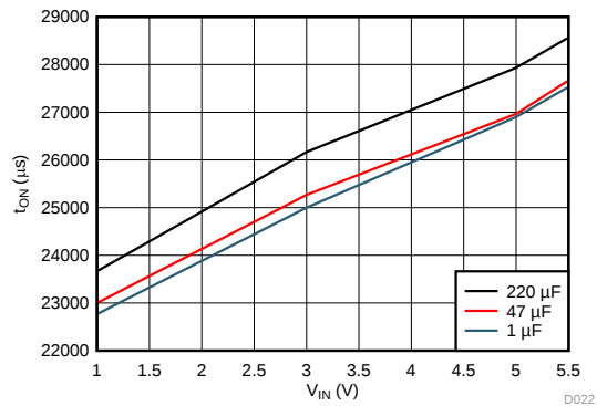
图 19. Turn On vs Load Capacitance (CT = 10000 pF)
