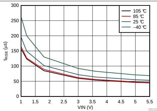
图 7. Turn On Time (CT = Open)
