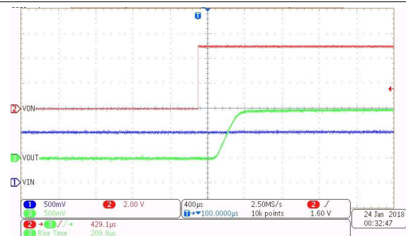
图 10. Turn On at 3.6 V (CT = Open)
