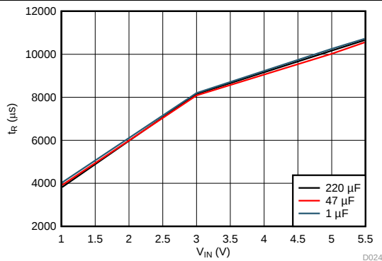
图 19. Turn On vs Load Capacitance (CT = 10000 pF)
