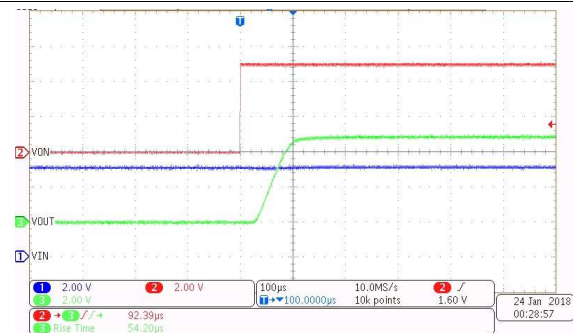
图 8. Turn On at 5 V (CT = Open)
