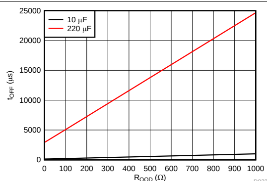
图 26. Turn Off at 3.6 V (Open Load)
