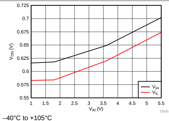
图 5. ON Pin Threshold
