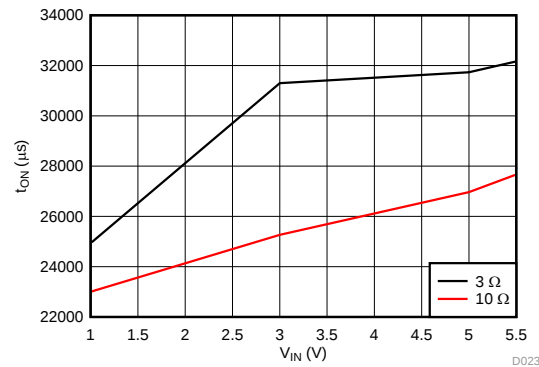
图 20. Turn On vs Load Resistance (CT = 10000 pF)
