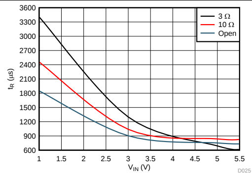
图 20. Turn On vs Load Resistance (CT = 10000 pF)
