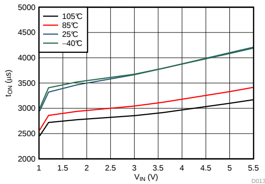
图 13. Turn On Time (CT = 1000 pF)
