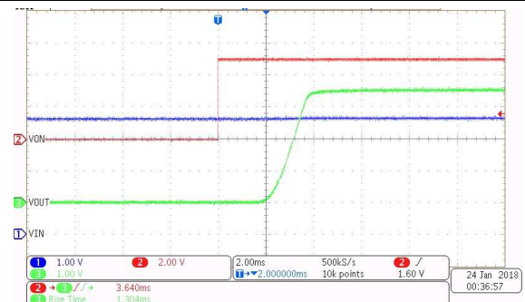
图 14. Turn On at 5 V (CT = 1000 pF)
