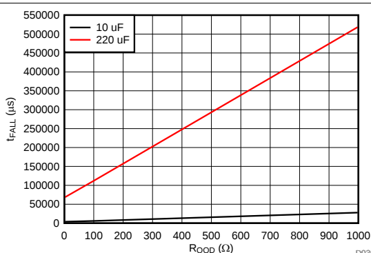
图 28. Turn Off Time (Open Load)
