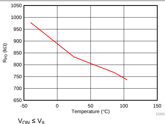
图 6. ON Pin Smart Pull Down ( R_{PD} )
