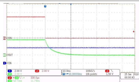
图 26. Turn Off at 3.6 V (Open Load)
