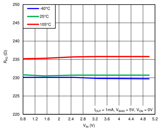
图 10. R_{PD} vs. V_{IN} ( V_{BIAS} = 5 V, Single Channel)
