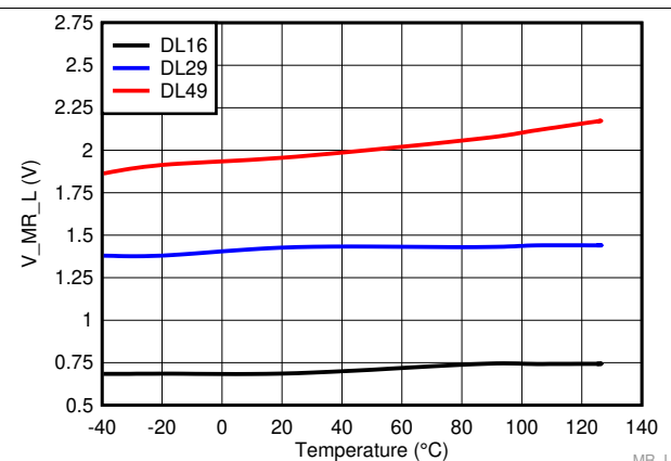
图 28. Manual Reset Logic Low Voltage Threshold over Temperature for TPS3840DLXX
