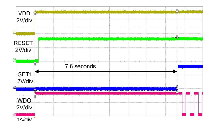
图 40. Startup Without a WDI Signal
