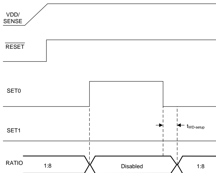
图 25. Enabling the Watchdog Timer
