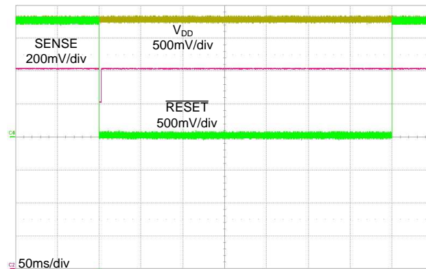
图 38. Typical \overline{\text{RESET}} Delay Timing
