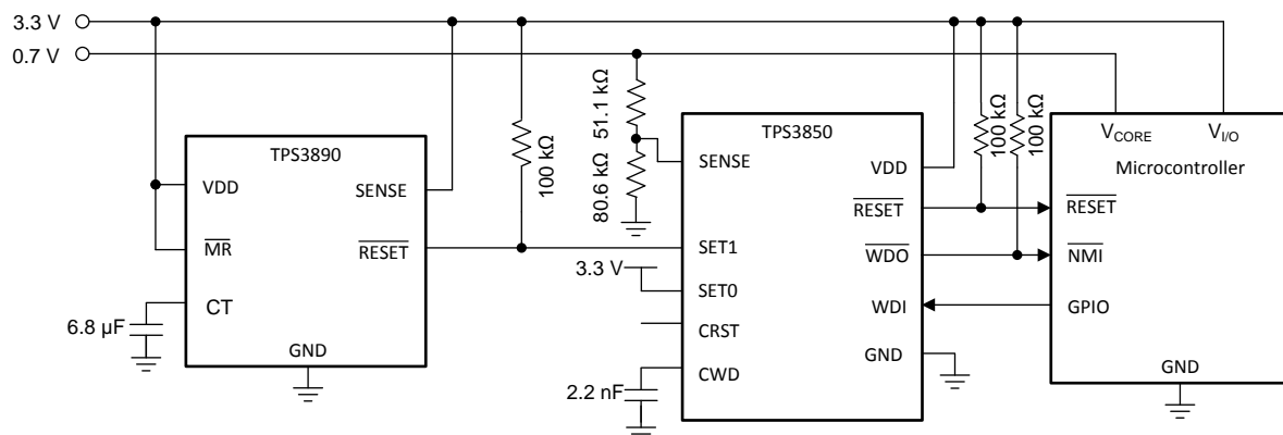
图 39. Monitoring Supply Voltage and Watchdog Supervision of a Microcontroller
