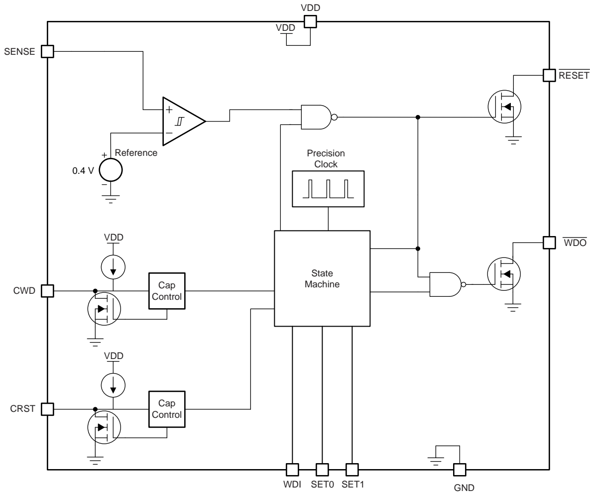
图 22. Adjustable Version Block Diagram
