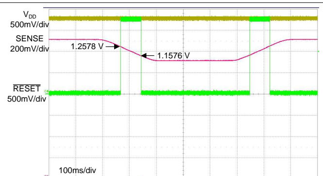
图 35. Window Comparator Thresholds Entering a Valid Window
