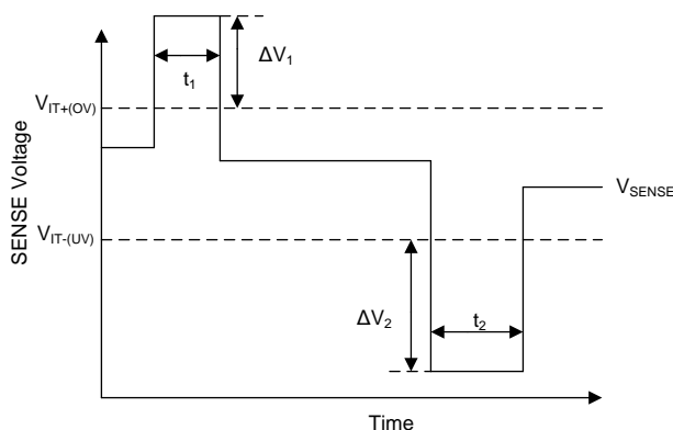
图 31. Overdrive Voltage on the SENSE Pin
