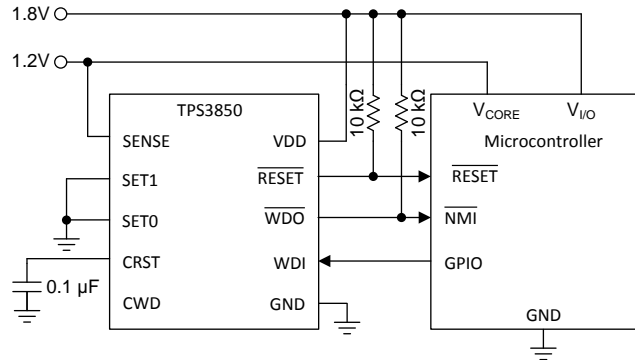
图 32. Monitoring Supply Voltage and Watchdog Supervision of a Microcontroller
