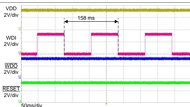
图 41. Typical WDI Signal
