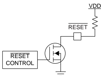
图 33. Open-Drain \overline{\text{RESET}} Configuration
