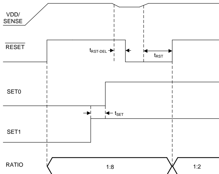
图 26. Changing SET0 and SET1 Pins
