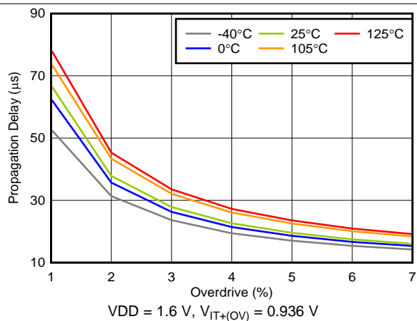
图 14. Propagation Delay vs Overdrive
