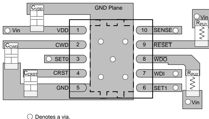
图 42. Typical Layout for the TPS3850
