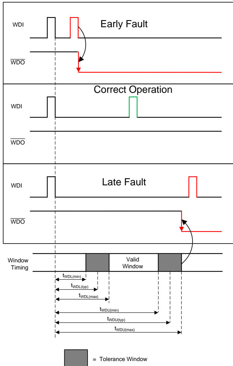
图 27. TPS3850 Window Watchdog Timing
