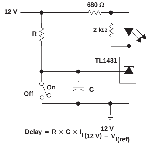
Figure 26. Delay Timer
