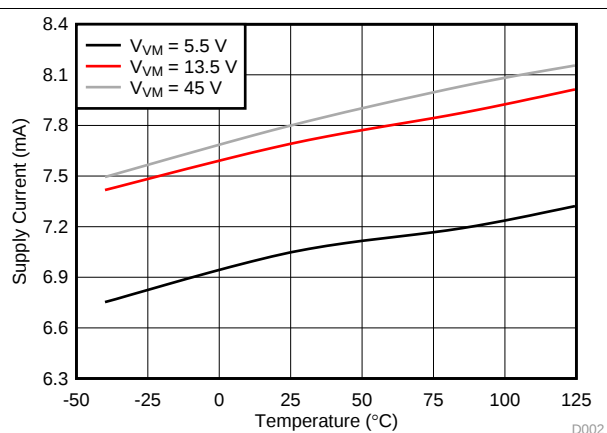
图 4. Supply Current vs Temperature
