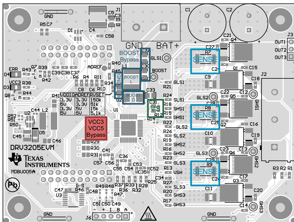
Figure 19. Layout Schematic
