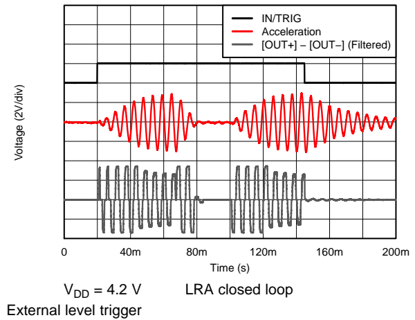
Figure 4. LRA Click With and Without Braking (RAM)
