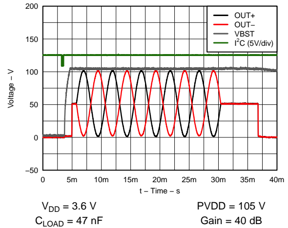
Figure 10. Typical Waveform
