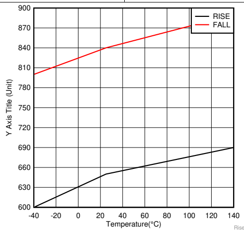
Figure 5. Rise And Fall Time with 1.8nC load
