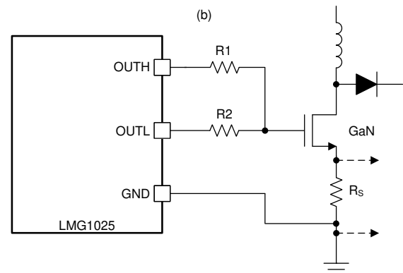
Figure 8. Source Resistor Current Sense B Configuration
