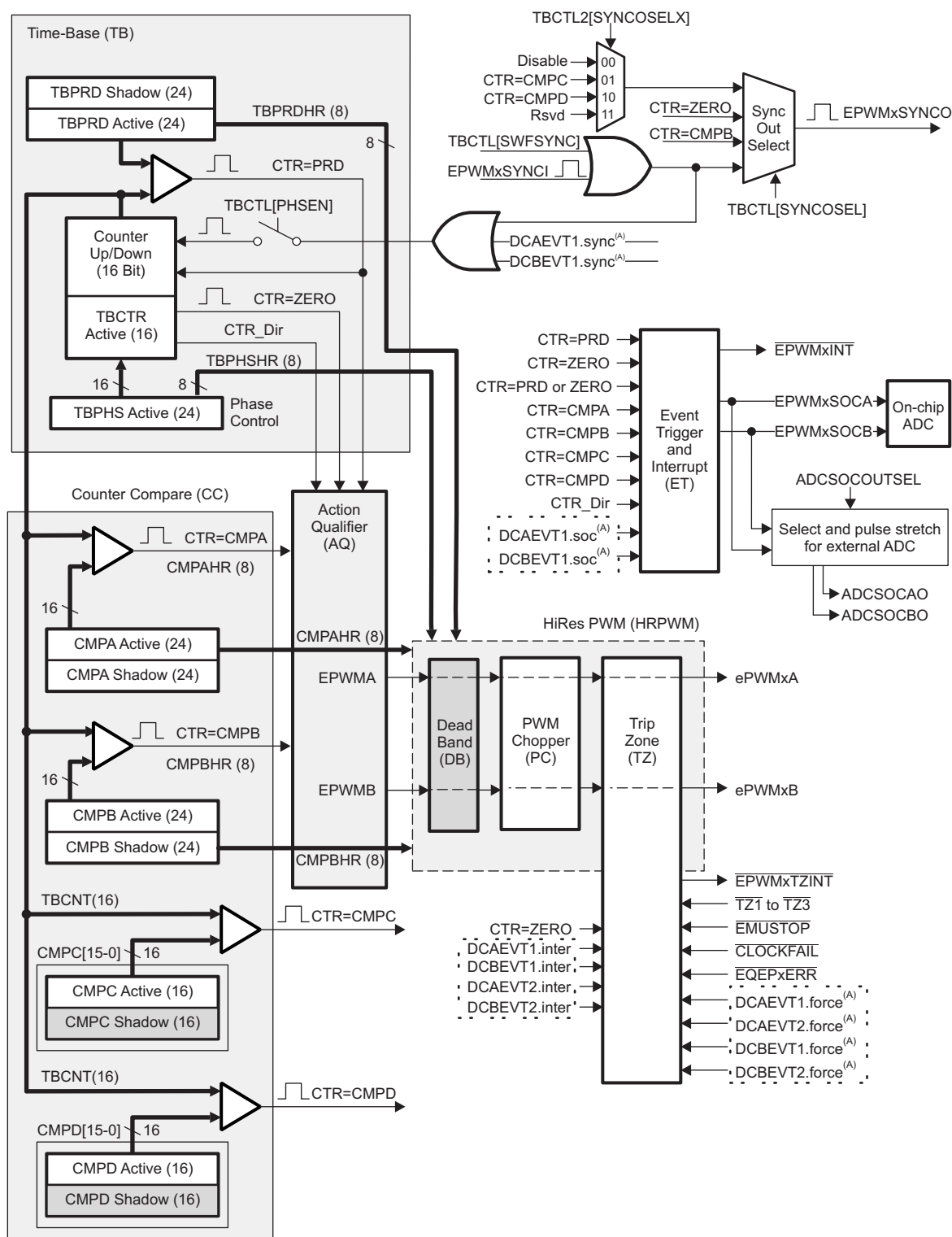
图 4-48. ePWM Submodules and Critical Internal Signal Interconnects
