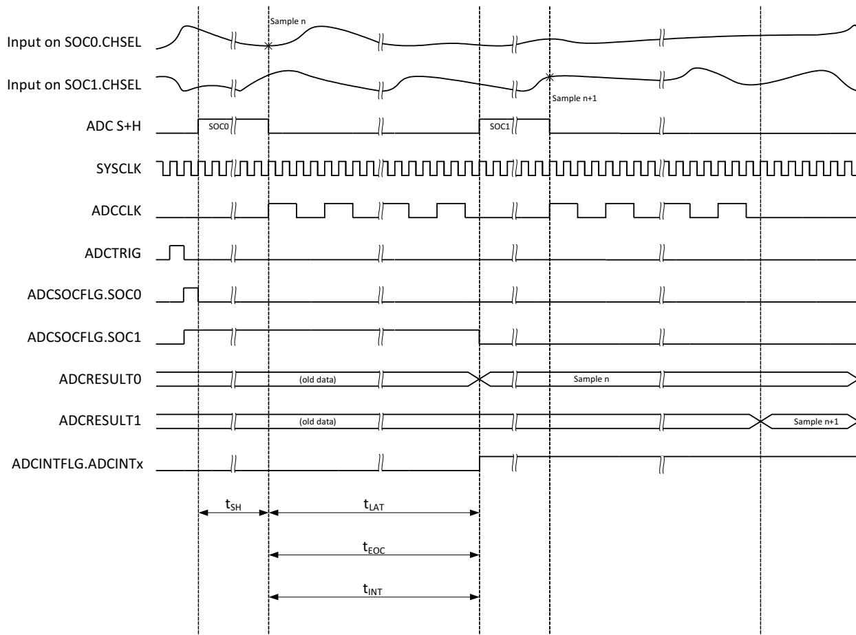
图 4-35. ADC Timings for 16-Bit Mode
