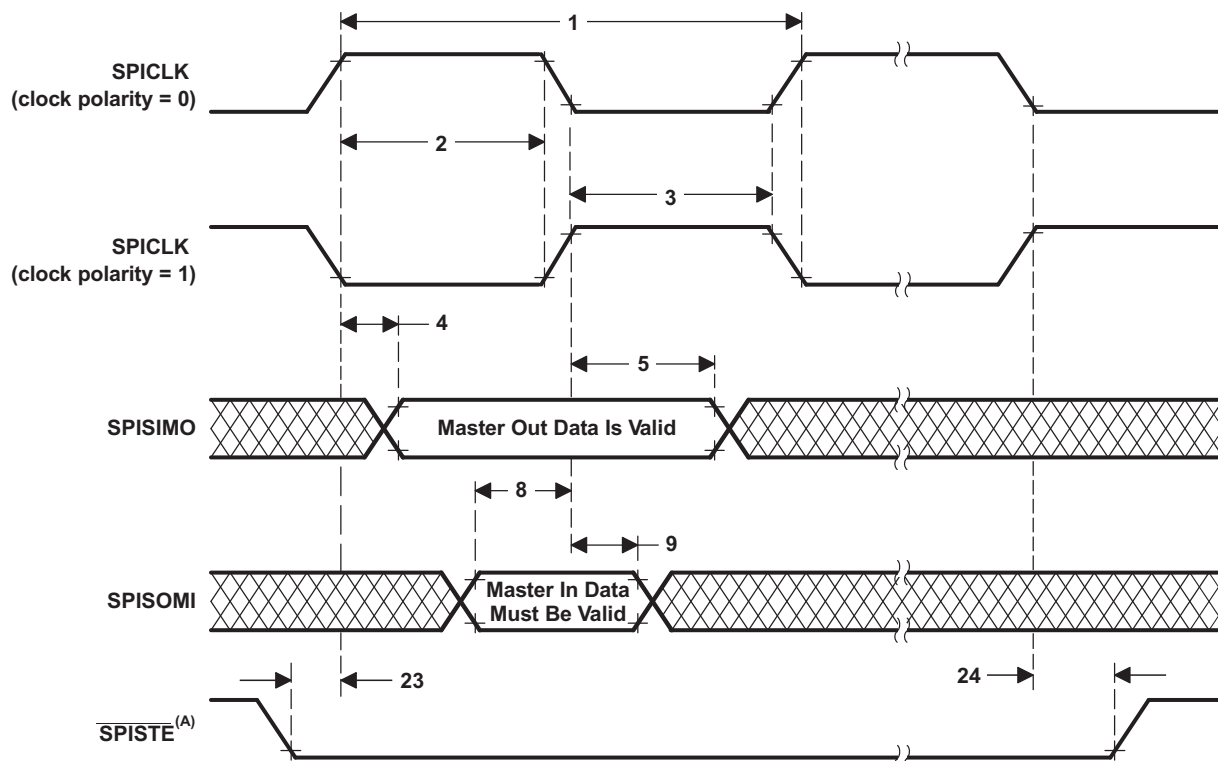
图 5-79. High-Speed SPI Master Mode External Timing (Clock Phase = 0)
