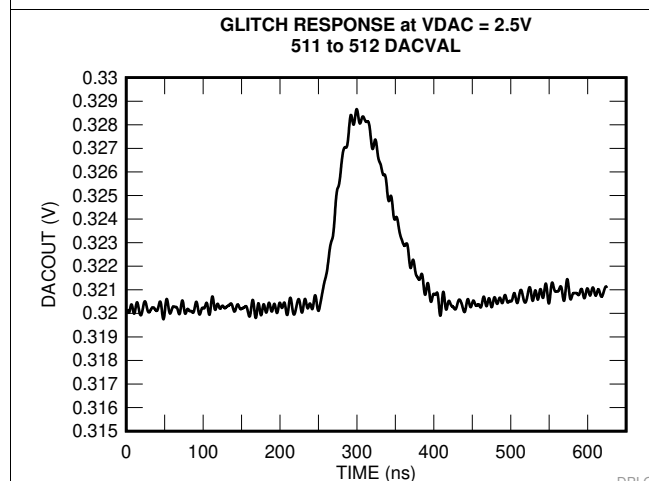
图 5-44. Glitch Response – 511 to 512 DACVAL
