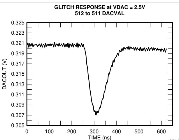
图 5-45. Glitch Response – 512 to 511 DACVAL
