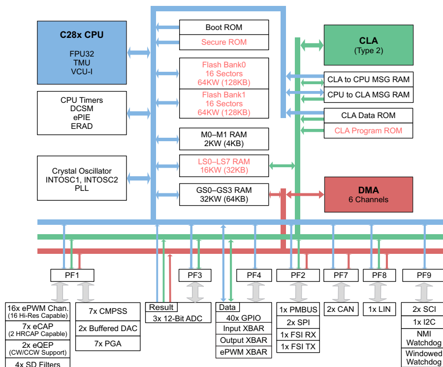
图 6-1. Functional Block Diagram
