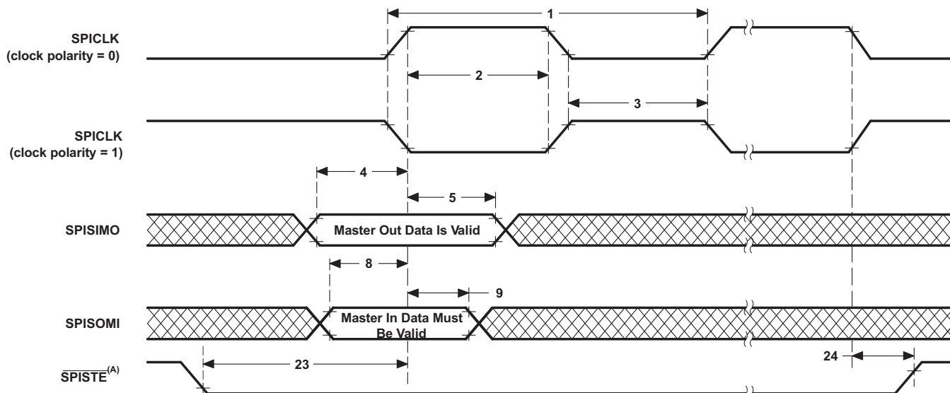
图 5-79. High-Speed SPI Master Mode External Timing (Clock Phase = 0)
