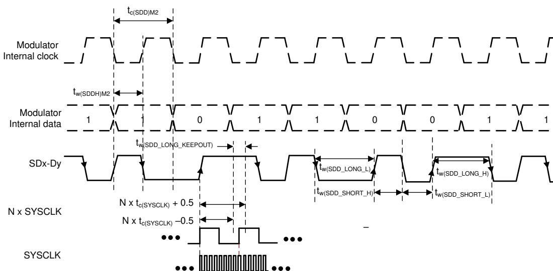
图 5-67. SDFM Timing Diagram – Mode 2
