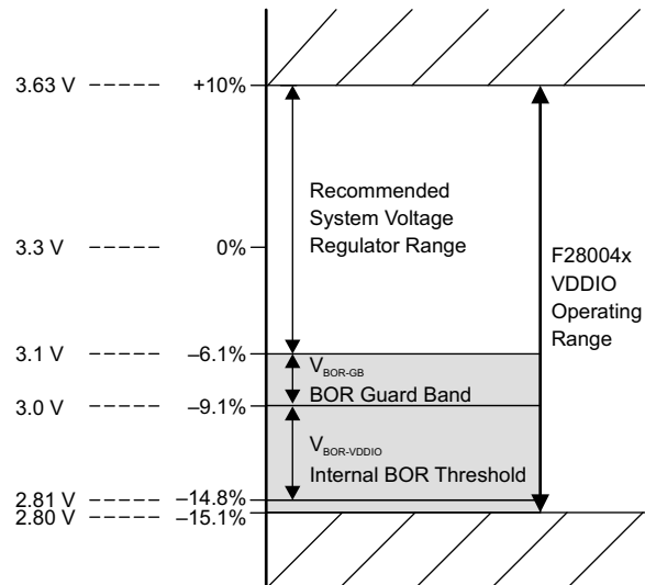
图 5-1. Supply Voltages
