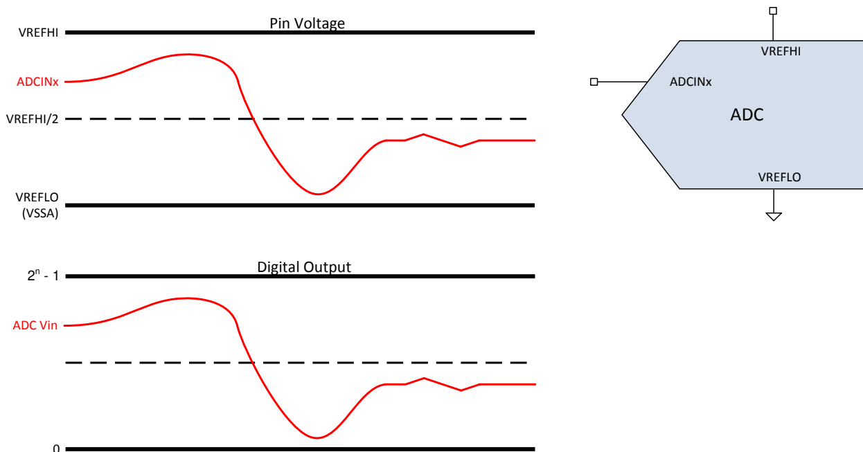
图 5-33. Single-ended Signaling Mode
