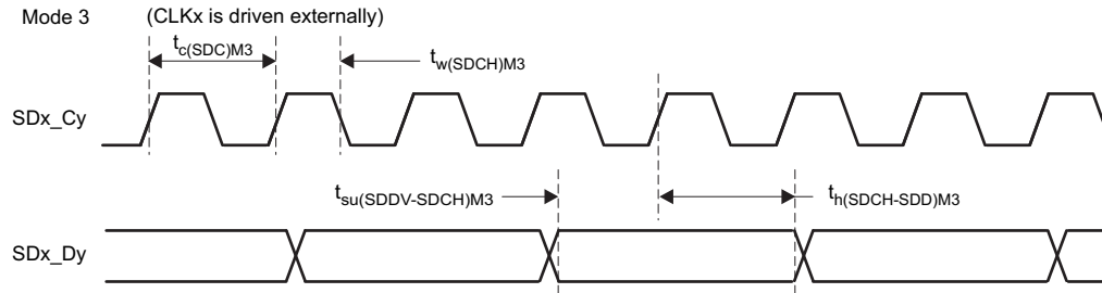
图 5-68. SDFM Timing Diagram – Mode 3
