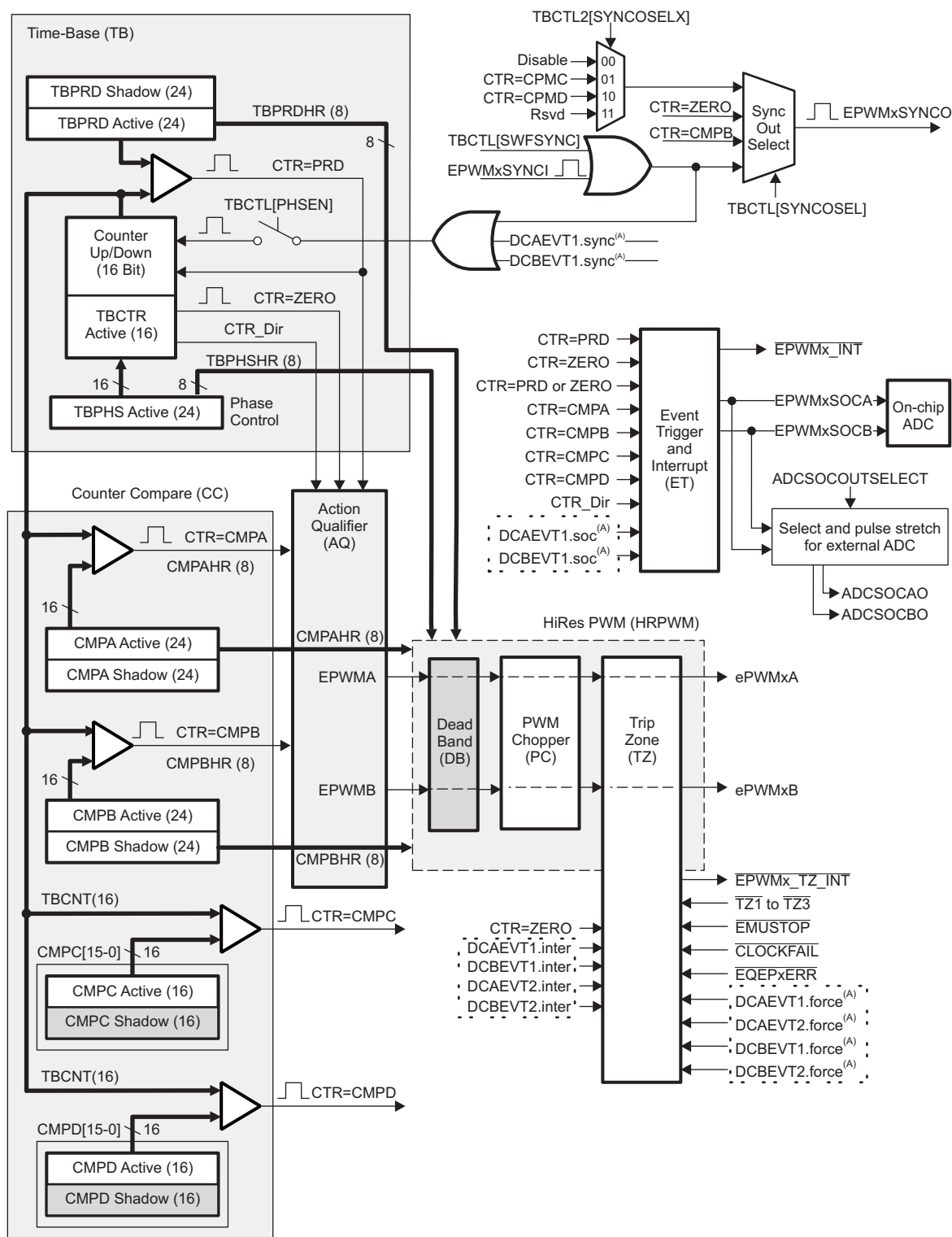
图 5-58. ePWM Submodules and Critical Internal Signal Interconnects
