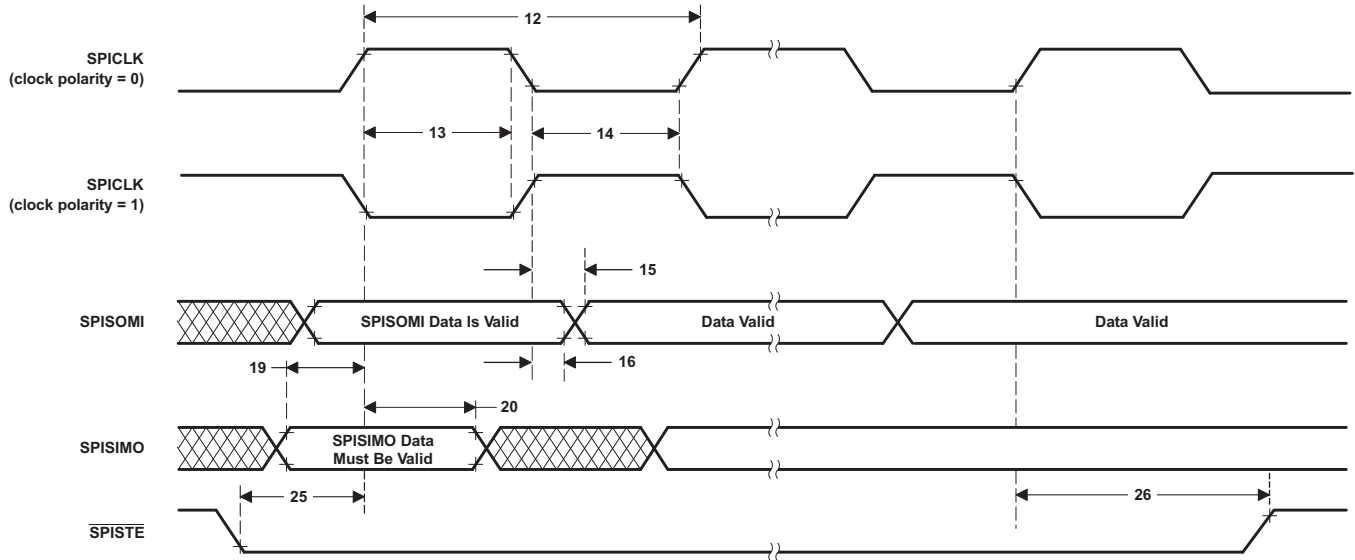
图 5-78. SPI Slave Mode External Timing (Clock Phase = 1)
