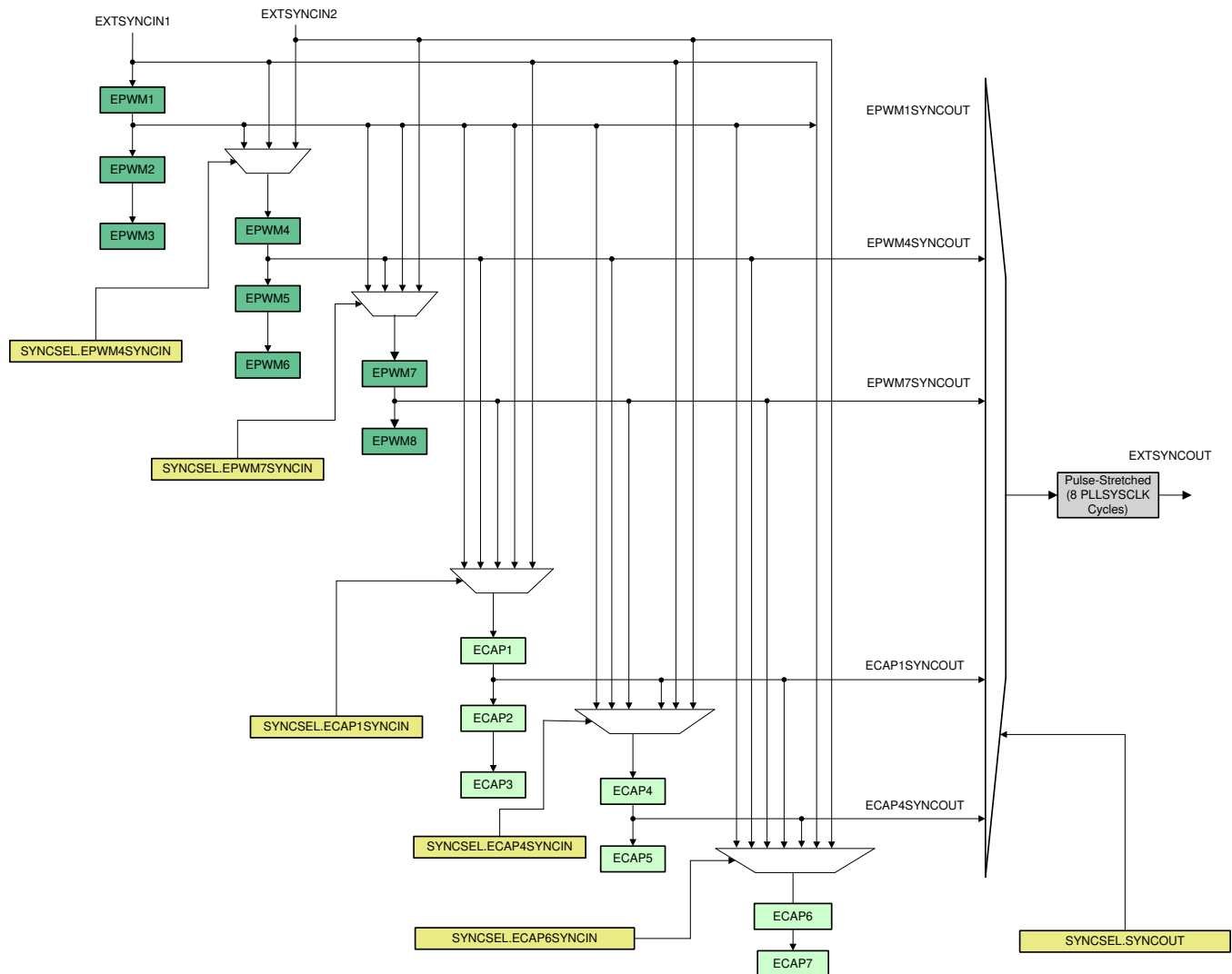
图 5-60. Synchronization Chain Architecture
