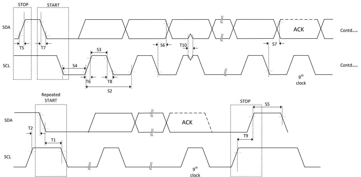
图 5-71. I2C Timing Diagram
