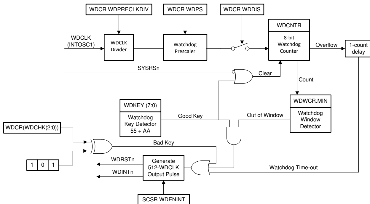
图 6-4. Windowed Watchdog
