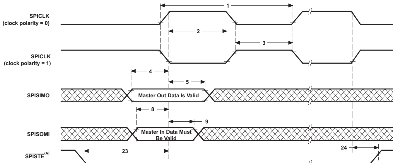
图 5-75. SPI Master Mode External Timing (Clock Phase = 0)
