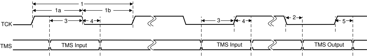
图 5-20. cJTAG Timing
