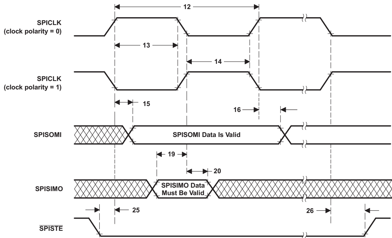
图 5-77. SPI Slave Mode External Timing (Clock Phase = 0)
