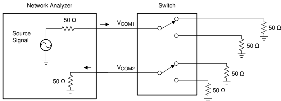
图 10. Cross Talk
