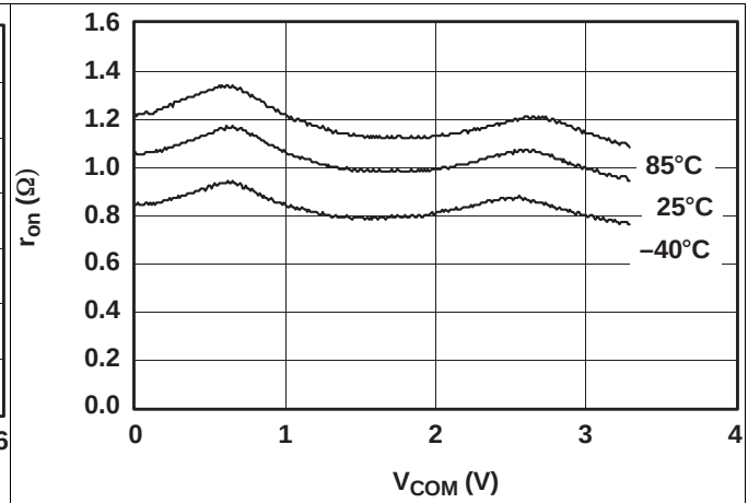
Figure 2. r_{on} vs V_{COM} ( V_+ = 3.3\text{ V} )
