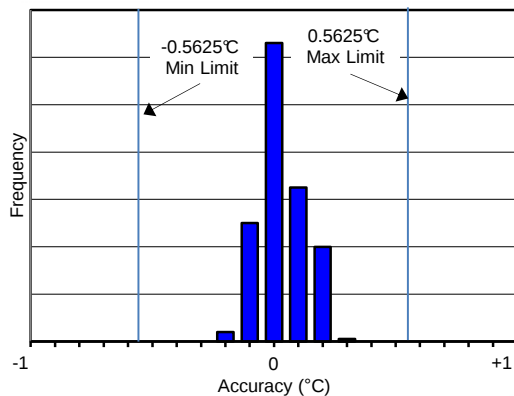
Figure 10. Accuracy Histogram at 30°C
