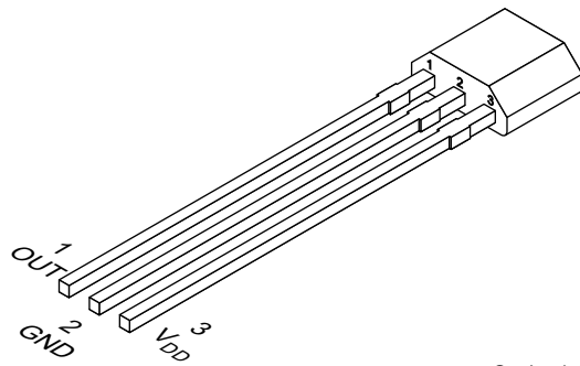
LPG Package 3-Pin TO-92S (Top View)
