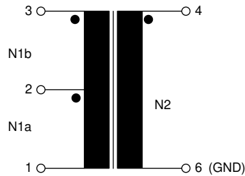
图 27. Typical Pinout of Center-Tap Transformer for Ultrasonic Transducers
