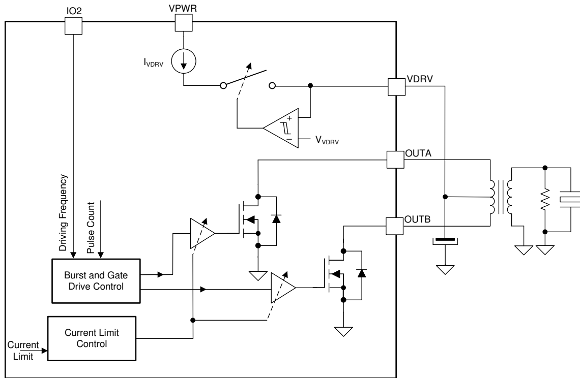
图 19. TUSS4440 Center-Tap transformer drive.
