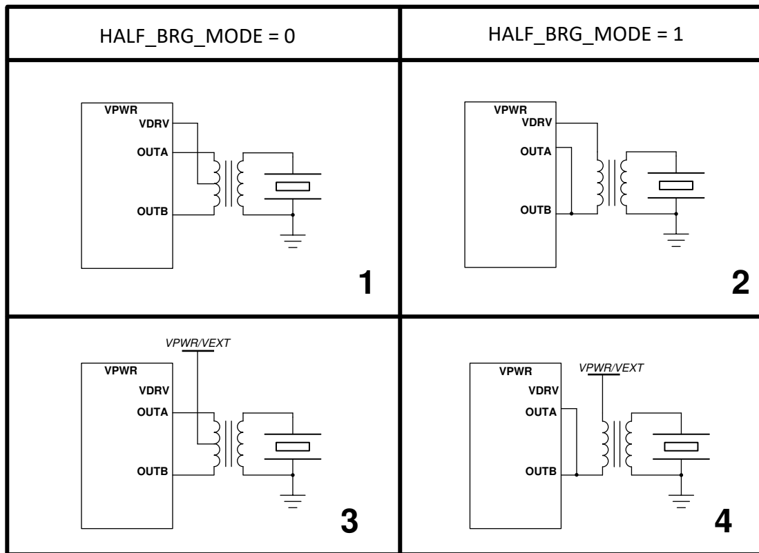
图 25. TUSS4440 Transducer Drive Options
