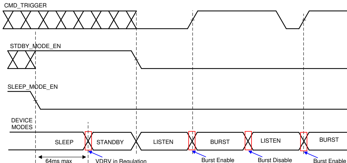
图 21. Device Modes Timing Diagram
