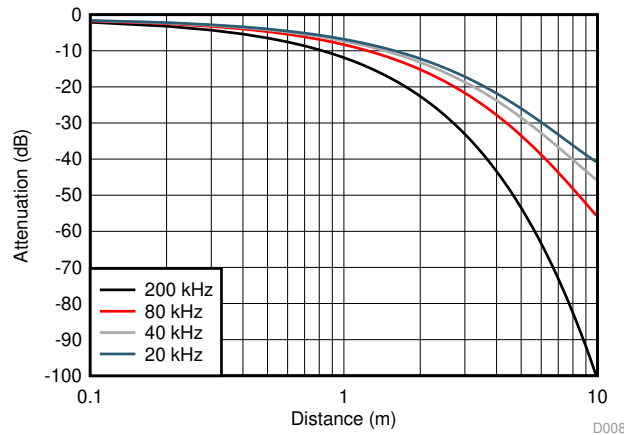
图 26. Attenuation Characteristics of Sound Pressure by Distance
